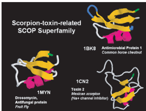
Fig. 1. Scorpion-toxin-related SCOP superfamily. These are only three members of a large superfamily including plant and insect defensins as well as scorpion toxins, provided as an example of the functional and structural diversity found in protein superfamilies. The N-terminus of each structure, shown in cartoon representation, is colored green, beta strands are colored yellow, helices are colored pink, hairpin turns are colored blue and loop regions are uncolored. These three proteins are believed to be related by divergent evolution from a common ancestor, and to share a common (albeit high-level) molecular function with obvious differences in specificity. Differences in structure are particularly evident in 1CN2, which has longer connecting and terminal loops, and only two helical turns compared with three in the other structures shown. BLAST comparison finds no recognizable sequence similarity between any two in this set, yet these are all part of a superfamily identified in the Structural Classification of Proteins database (see http://scop.berkeley.edu/data/scop.b.h.d.h.html ).
