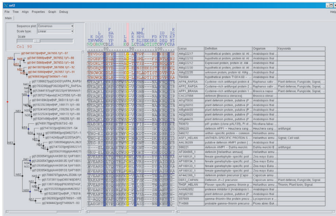
Fig. 3. GTREE software for phylogenomic analysis. Shown above is the GTREE user interface created by our group to correlate a phylogenetic tree with a multiple sequence alignment and experimental data. Data shown in the table are downloaded automatically from GenBank and SwissProt. Columns in the spreadsheet can be resized, re-ordered, inserted and modified. Subtrees can be viewed separately, removed from the tree, or collapsed to view a consensus sequence and consensus attributes. The GTREE software is available for UNIX/Linux platforms, and can be downloaded from the Berkeley Phylogenomics Group website at http://phylogenomics.berkeley.edu/software/ . New user interfaces written in Java are under development by our group; these will also integrate protein structure visualization and analysis.
