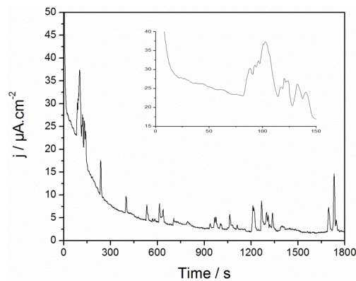
Figure 12. Current transient for AA5083-H116 obtained at 25mV below E_{\text{pit}} . Inset shows a zoom of a region of interest that represents the typical transient features (adapted from(Gupta, Sukiman et al. 2012))
