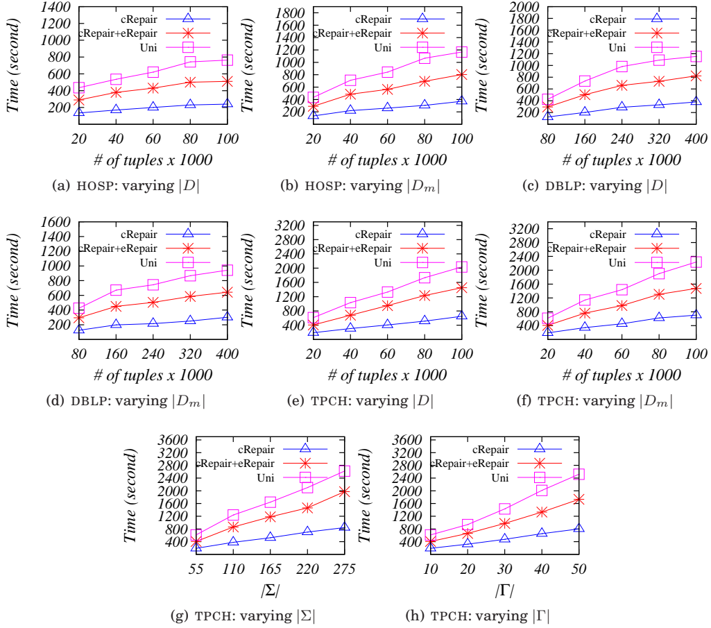
Fig. 14. Experiment 5: Scalability
