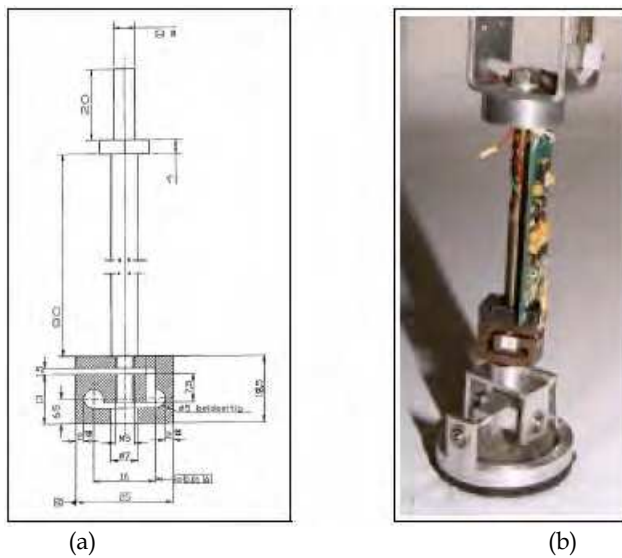
Fig. 3.3. Design of three-component force sensor.
