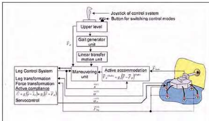
Fig. 4.1. Block-scheme of control system.
