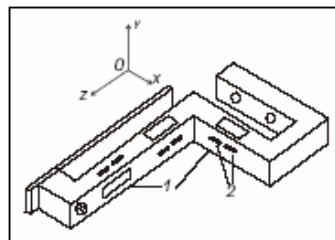
Fig. 3.4. Three-component force sensor composed of parallelogram element.
