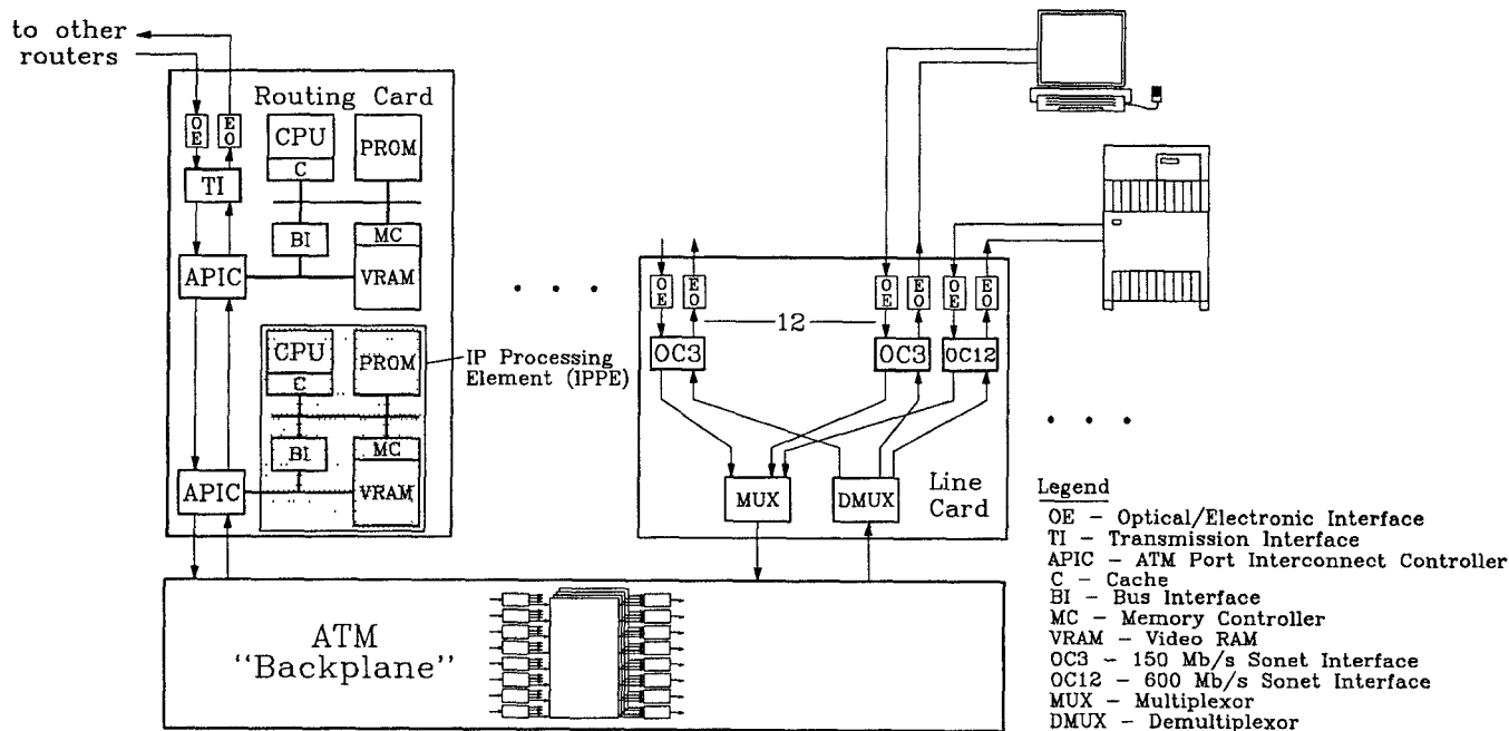
Figure 1: Gigabit a t Pm Router
