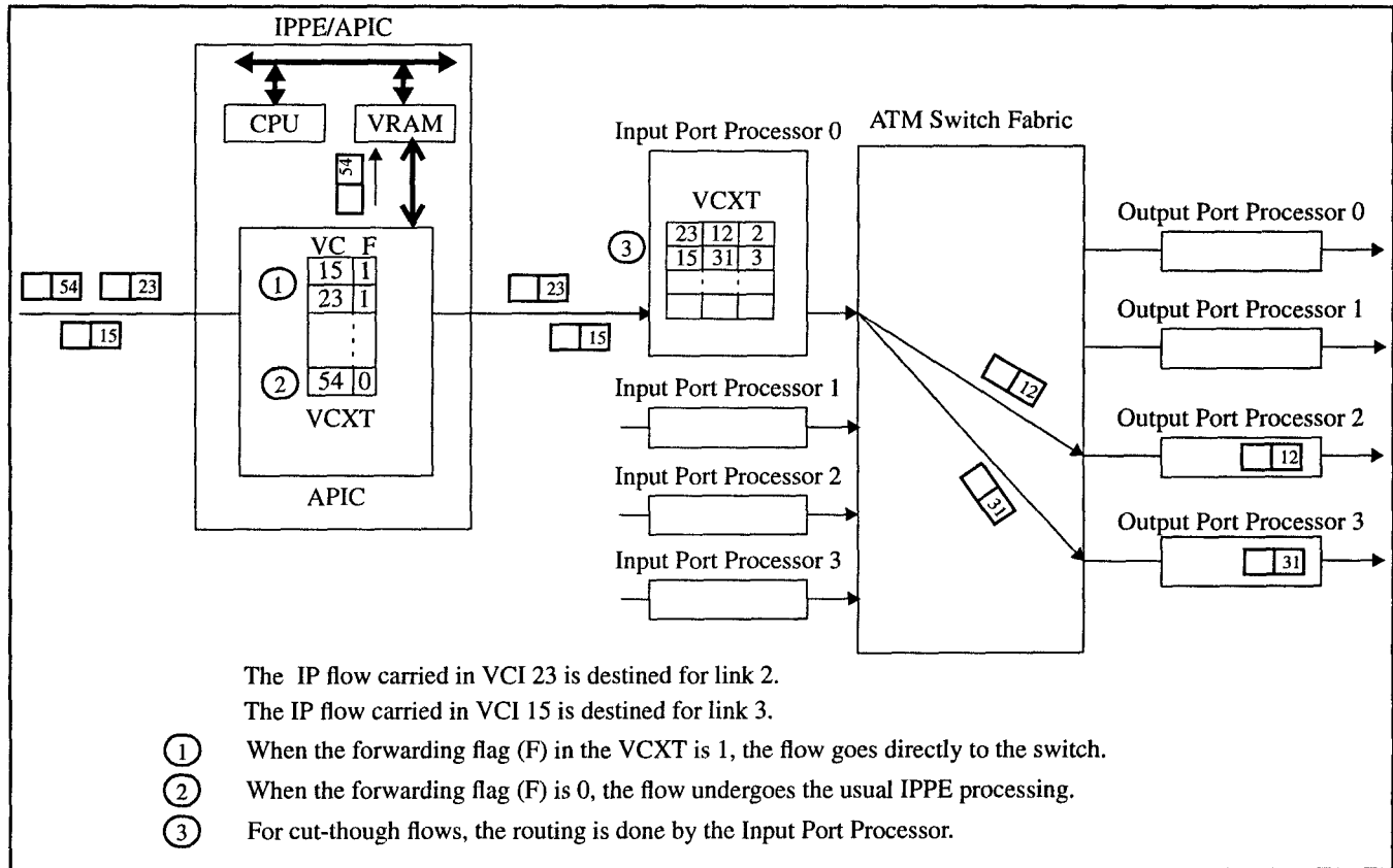
Figure 6: Cut-through Routing
