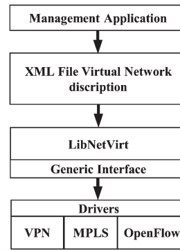
Fig. 13. LibNetVirt architecture.
