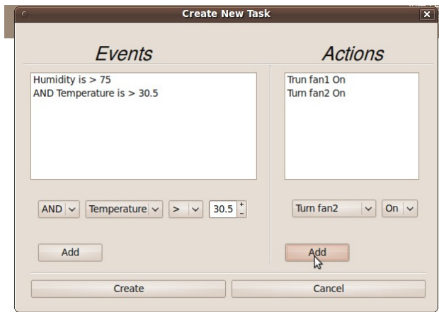
Fig. 5. Rule creator view.
