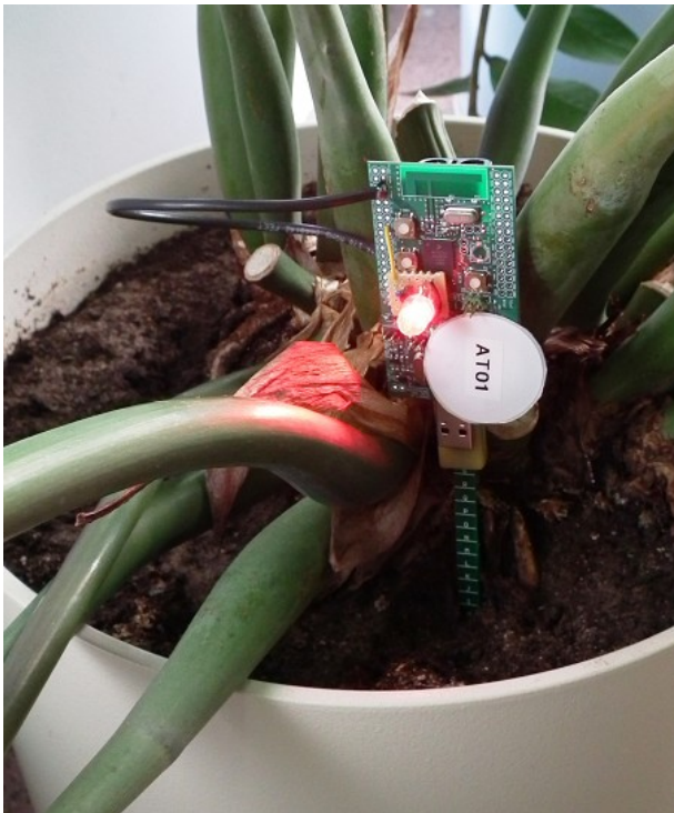
Fig. 3. Active tag in a potted plant.
