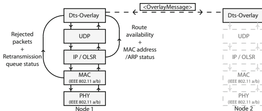
Fig. 1. Cross-layer Information Flow in Dts-Overlay
