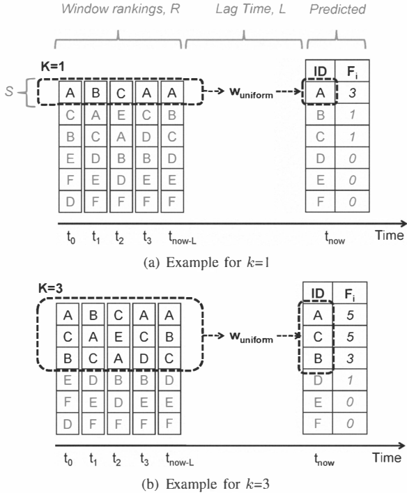
Figure 2. Example of the top- k set membership prediction problem, using uniform weighted frequency selection.
