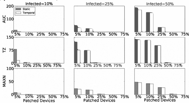
Figure 8. MIT: Effects of increasing number of patched devices against initial infected devices. Midday infection, 3 hours patch delay.
