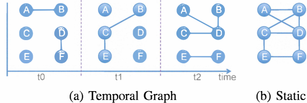
Figure 1. Example (a) temporal graph and corresponding (b) static graph.
