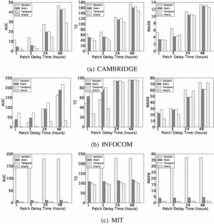
Figure 6. Best centrality prediction binned by patch delay (upload interval 24 hours).
