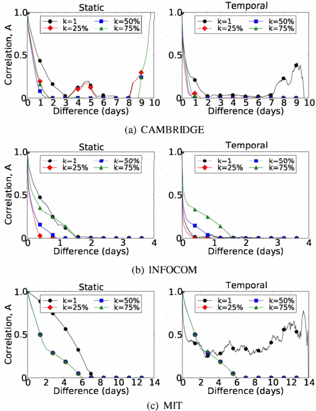
Figure 3. Plotting self similarity between the rankings related to all windows a with all windows b \leq a , averaged by time difference d = a - b (x-axis). Static (left column) and temporal (right) centralities plotted. Legacy correlation is observed with both static and temporal centrality.
