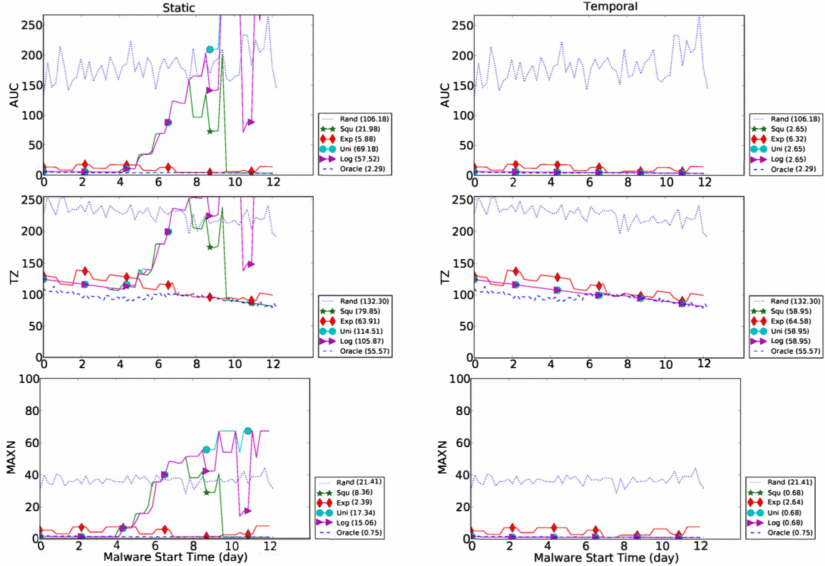
Figure 5. MIT Traces: Comparison of Centrality type vs. Prediction Function, as a function of Start Time (x-axis).
