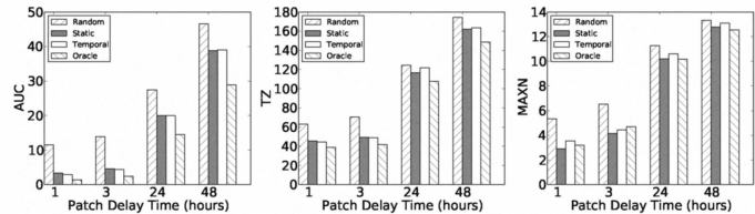
Figure 7. CAMBRIDGE: Best centrality prediction binned by patch delay (upload interval 1 hour).
