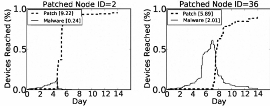
Figure 4. MIT: Malware started at day 0 and patch started 1 day later from device selected by temporal closeness (left) and random (right). Area under each curve reported in legend.
