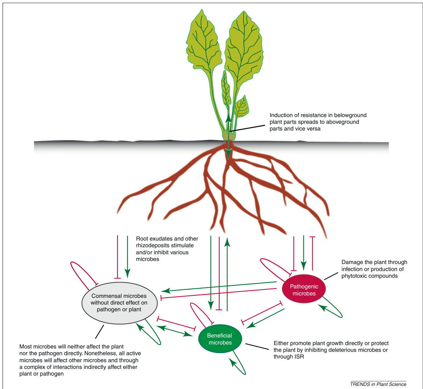
Figure 2. Interactions in the rhizosphere. Plants are able to influence the composition and activation of their rhizosphere microbiome through exudation of compounds that stimulate (green arrows) or inhibit (red blocked arrows). Vice versa, a wide range of soil-borne pathogens are able to affect plant health. Prior to infection, these deleterious microbes are in competition with many other microbes in the rhizosphere for nutrients and space. In this battle for resources, beneficial microbes will limit the success of the pathogen through production of biostatic compounds, consumption of (micro)nutrients or by stimulating the immune system of the plant. Most microbes might neither affect the plant nor the pathogen directly because they occupy different ecological niches (commensal microbes), but are likely to affect every other organism to a certain extent through a complex network of interactions. Abbreviation: ISR, induced systemic resistance.
