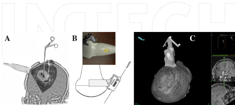
Figure 1. Ultrasound-based guidance: A) Freehand guidance: challenge to have the long axis of the instrument in the 2D ultrasound plane. B) Needle guides: an adapter mounted on the probe makes sure that the instrument is within the 2D ultrasound plane. C) Navigation: tracking technology and 3D data from modalities like CT, MR and ultrasound is used to guide relevant surgical instruments in place. Here an ultrasound probe is guided by MR during a freehand 3D ultrasound acquisition
