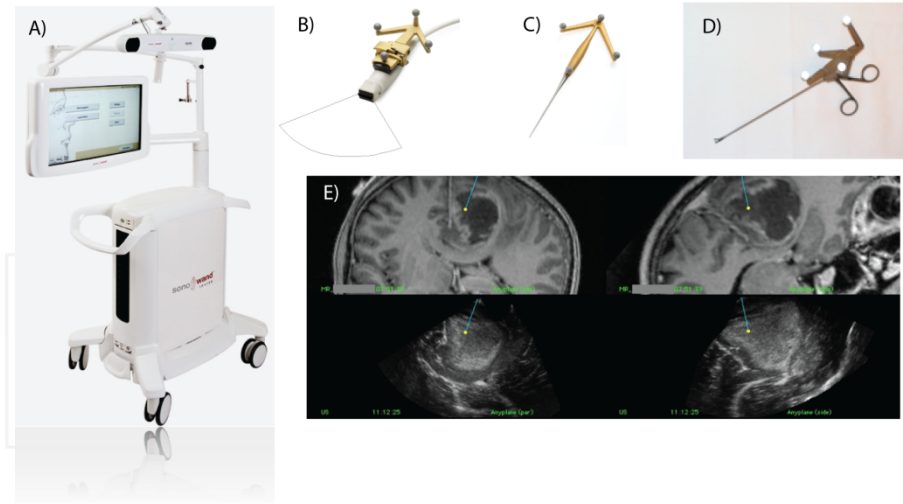
Figure 21. The Sonowand Invite® system for intraoperative ultrasound imaging and navigation (A), various tools of the navigation system equipped with optical localizer units showing one phased array ultrasound probe (B), a navigation pointer (C), a biopsy forceps (D), and a screen dump of the navigation display showing reformatted MR images in top row, and corresponding reformatted ultrasound images in bottom row (E). The tip of the navigated instrument is indicated with a bright spot in the reformatted image slices
