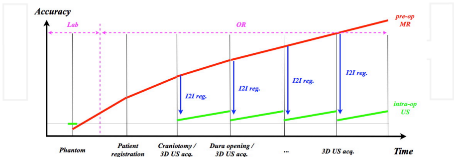
Figure 19. Navigation System Accuracy (NSA) based on preoperative (p) MR (red line) and intraoperative (i) US (green line). iUS can be used to correct pMR using various image-to-image registration techniques (blue line).
