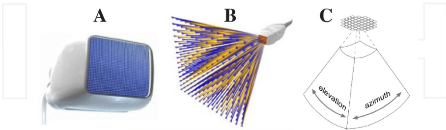
Figure 12. Matrix probes. Using a 2D array of elements (A) the beam can be steered in two directions (B) and a truncated pyramid of data is acquired (C).
