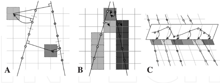
Figure 10. Reconstruction methods: A) Voxel Nearest Neighbor (VNN), B) Pixel Nearest Neighbor (PNN), Distribution Step (DS) and C) Functional Based Methods (FBM).
