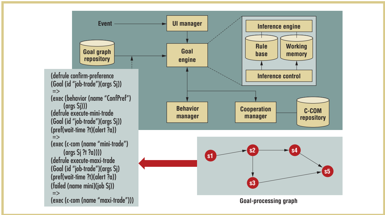
Figure 2. A goal-achieving process for cooperative service provision.
