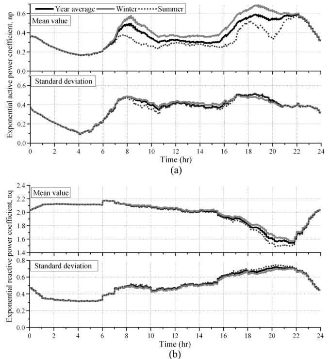
Fig. 6. Comparison between load model coefficients for characteristic loading conditions.
