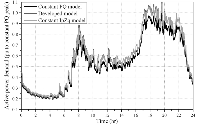
Fig. 7. Aggregate power demand for detailed model and constant PQ model for maximum voltage conditions.
