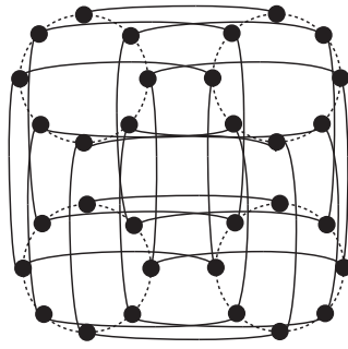
Fig. 1. Four cycles connected in the shape of a cycle.
