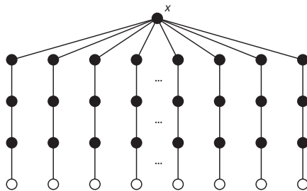
Fig. 2. An extended star rooted at x .
