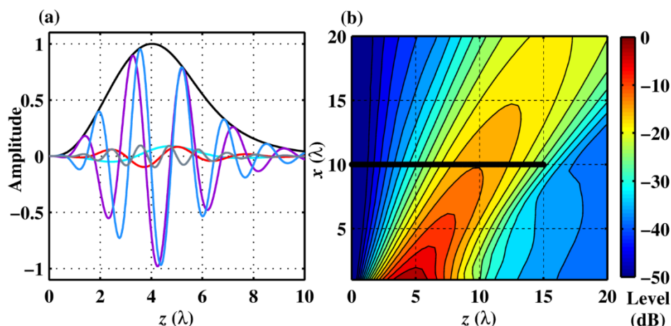
Fig. 1 (a) Wavepacket magnitude and associated real parts for a source distribution consisting of multiple wavepackets with varying wavenumber. (b) The resultant radiated field and a black line indicating the array input for the beamforming algorithms.
