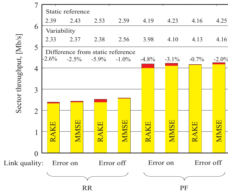
Figure 5.5: Effect of other-sector interference variability in the 1 \times 1 SISO case, under the OWNP2 model, in PeA and in combination with an activity factor \alpha of 0.5.
