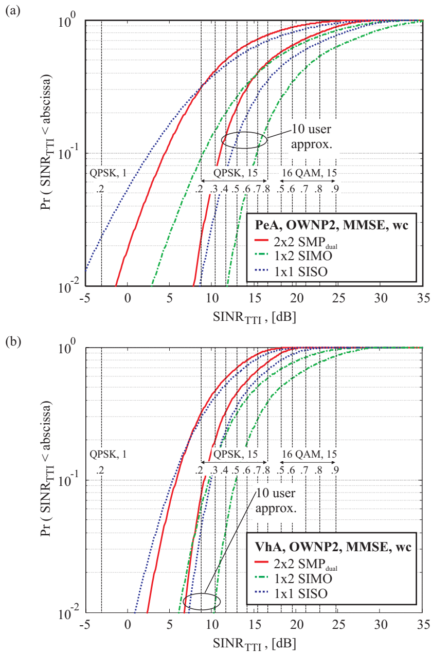
Figure 5.18: 2 \times 2 SMP_{\text{dual}} SINR statistics as encountered over the whole sector area in (a) PeA and (b) VhA. 1 \times 1 SISO and 1 \times 2 SIMO serve as reverences.
