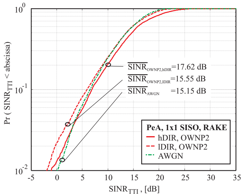
Figure 5.3: Influence of DIR on SINR distribution.
