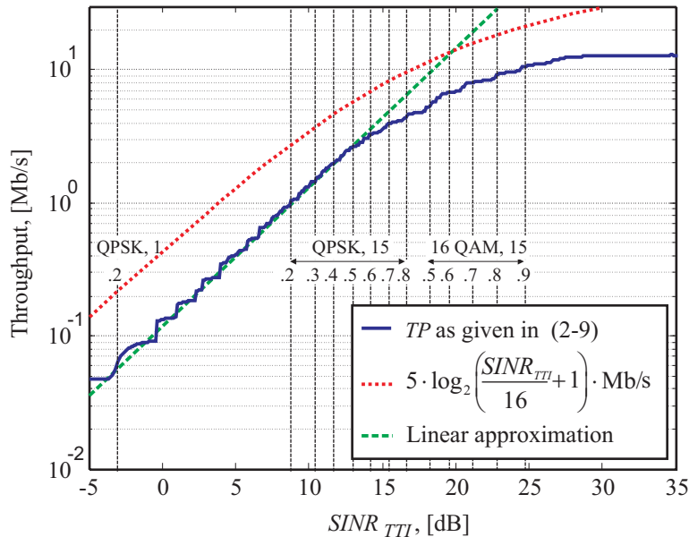
Figure 2.5: SINR-to-throughput relationship.
