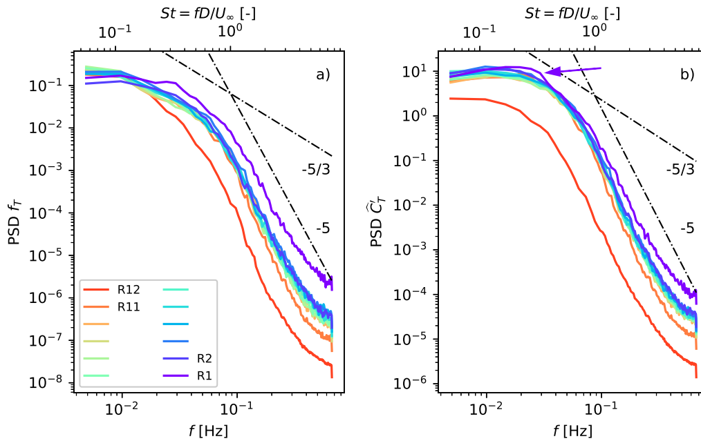
Figure 7. Power spectral density (PSD) estimates of the row-averaged thrust force f_T (a) and thrust coefficient \hat{C}_T^i (b) as a function of frequency f (bottom axis) and non-dimensional Strouhal number St (top axis).
