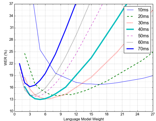
Figure 1: Word Error Rate (%) versus Language Model Weight for various frame durations.
