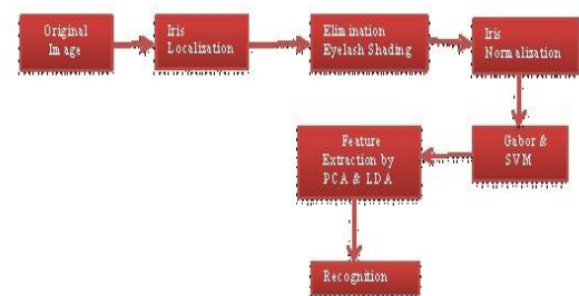
Fig 1 Proposed Algorithm
