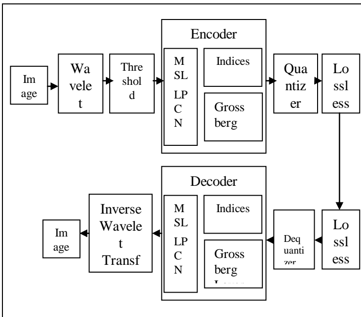
Fig. 6 Block Diagram for Wavelet – CPN Based Image Compression
