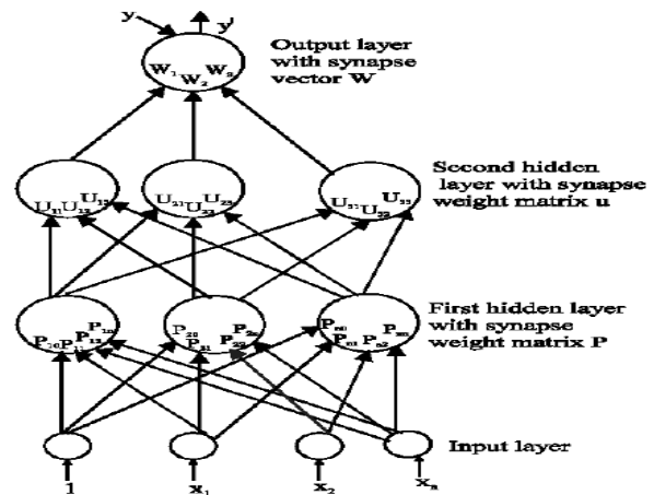
Fig 3: Structure of Two hidden Layer Network
