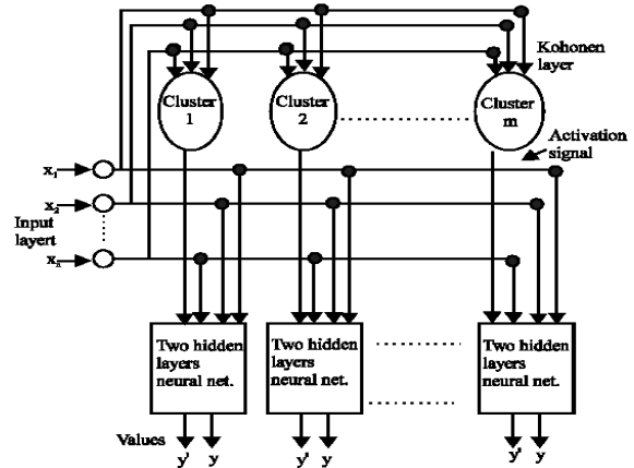
Fig 2: Modified Single Layer Linear Counterpropagating network
