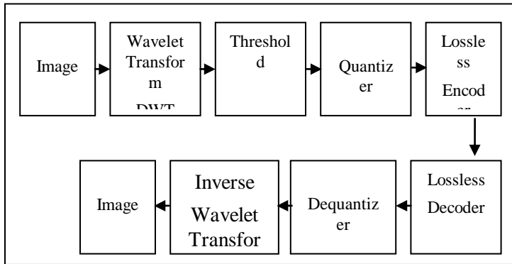
Fig. 5 Block Diagram for Wavelet Based Image Compression
