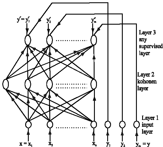
Fig.1 The Forward Only Counter propagation network
