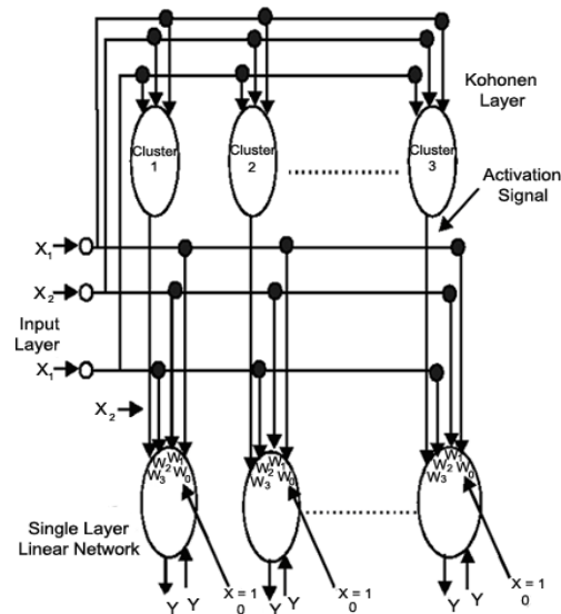
Fig.4: The final structure of SLLIC Network
