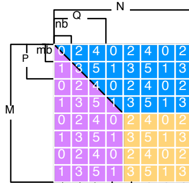
Figure 17: Block cyclic distribution of a 8m_b \times 8n_b matrix over a 2 \times 3 process grid.
