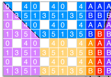
Figure 20: Single failure during a Q -panel update of the ABFT LU factorization.
