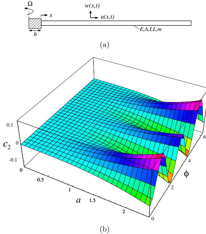
Figure 19: First flapping NNM of a rotating beam. (a) Schematics of the system; (b) slave modal coordinate c_2 corresponding to the second flapping mode. Figure reproduced from [124].
