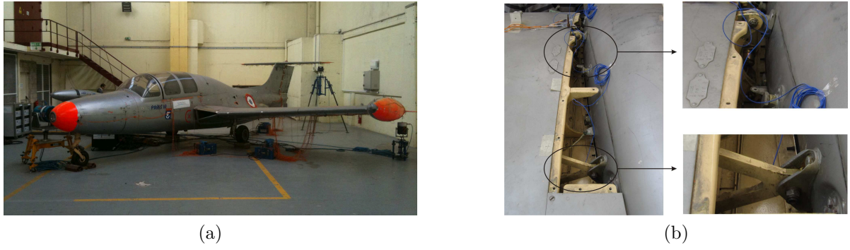
Figure 5: Morane-Saulnier 760 aircraft. (a) Photograph; (b) close-up of the bolted connections between the wing tip and an external fuel tank. Figure reproduced from [68].
