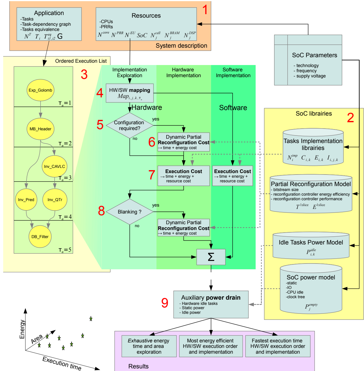
Fig. 4. Global exploration and power / performance estimation flow.
