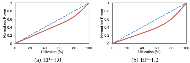
Figure 8. EP curve for Peak Efficiency Aware Scheduling
