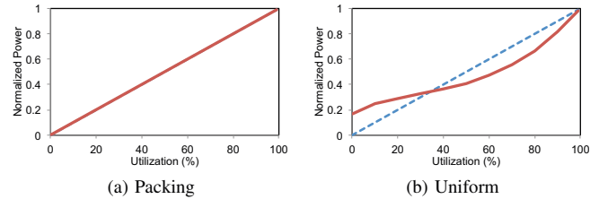
Figure 6. Best case cluster-wide energy proportionality curve for various cluster-level load balancing schemes (red solid line). The blue dotted line represents linearly ideal energy proportionality.
