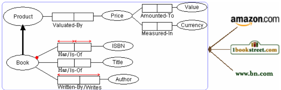
Fig. 1. Ontology A
