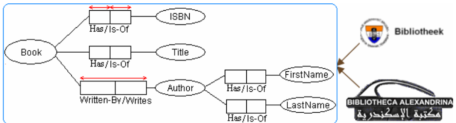
Fig. 2. Ontology B
