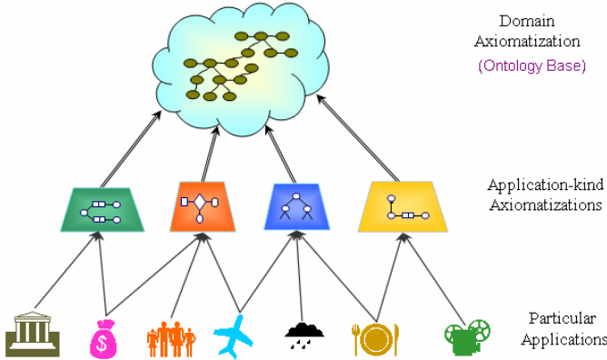
Fig. 3. DOGMA framework
