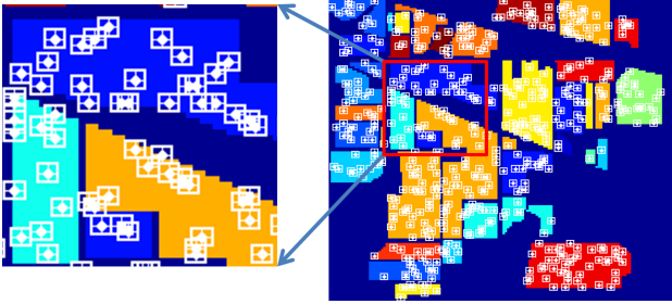
Fig. 5. Overlap between training and testing data on Indian Pine dataset under 5% sampling rate.
