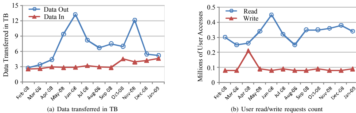
Fig. 4. The amount of data written/read to/from and the number of read/write requests issued to the Internet Archive servers as a function of time during a one-year period.
