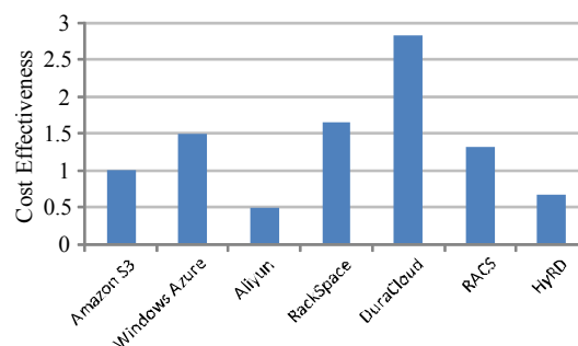
Fig. 9. Benchmark results on cost effectiveness of the different schemes. Note that the lower the value, the better for the cost effectiveness.
