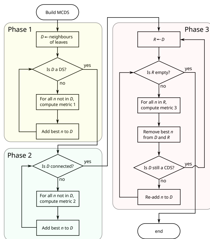
Figure 1. Flowchart for the computation of the minimum connected dominating set (MCDS).
