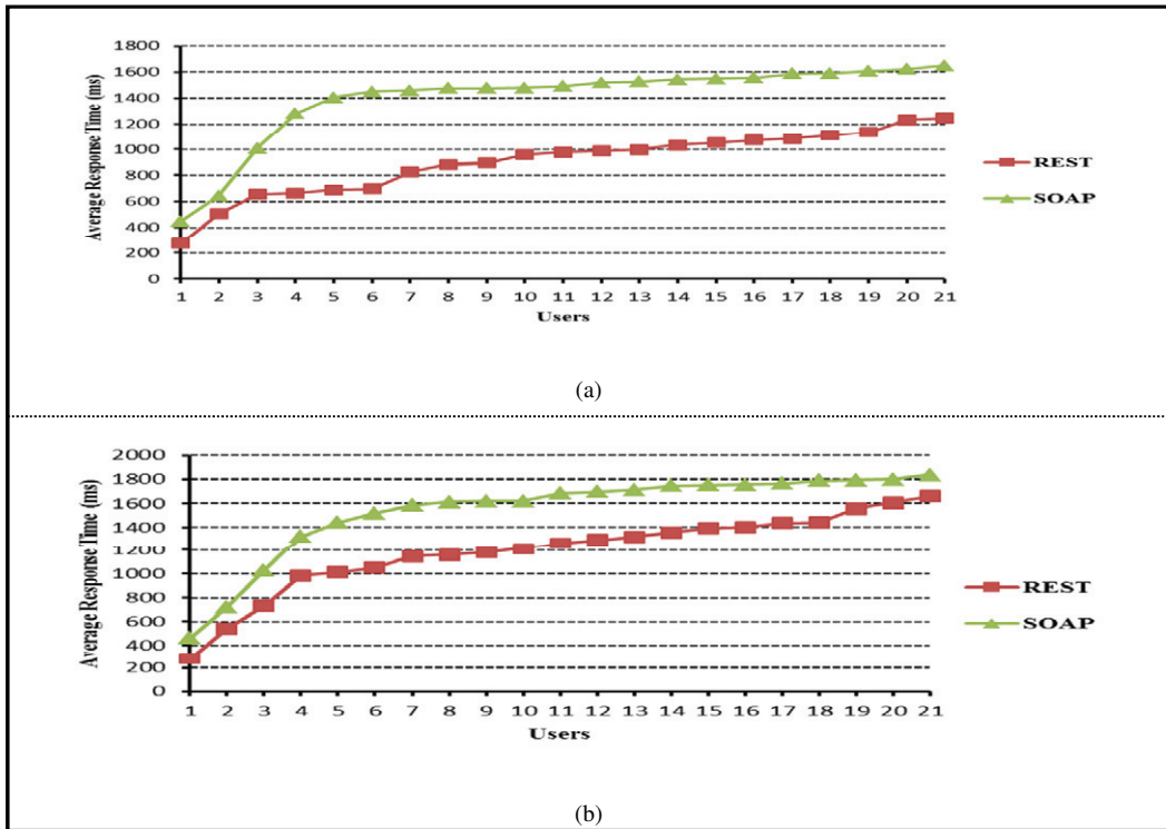
Figure 4. Mobile host average response time for SOAP-based and RESTful web services during concurrent (a) HTTP GET requests; (b) HTTP PUT requests.
