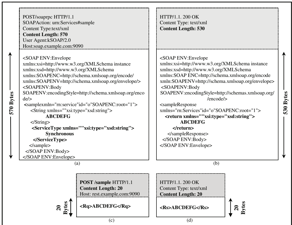
Figure 1. Sample SOAP web service (a) request; (b) response compared to sample RESTful web service (c) request; (d) response.
