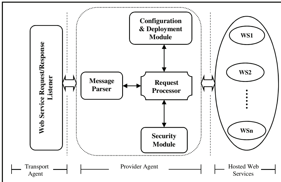
Figure 2. Framework building blocks for mobile web services host.
