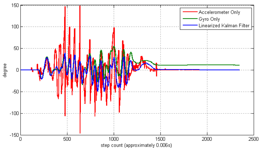
Fig. 4. Unsteady motion measurement using Kalman filter.
