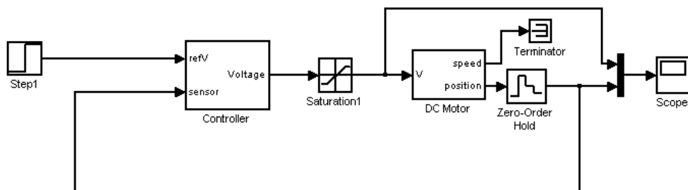
Fig. 5. Block diagram for motor position control.
