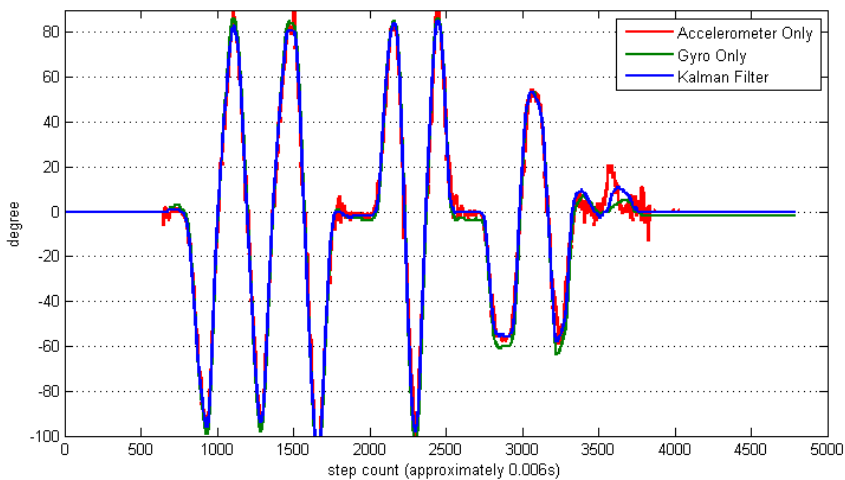
Fig. 3. Steady motion using Kalman filter.
