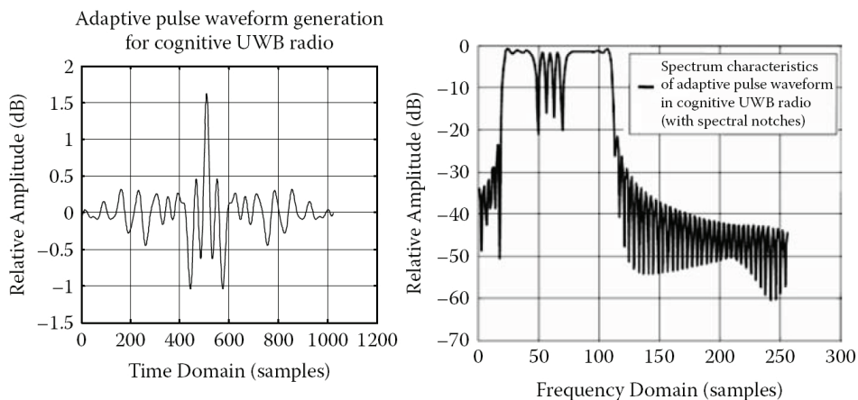
Fig. 5. Adaptive pulse waveform with spectrum-agile characteristics (Zhang et al., 2009)
