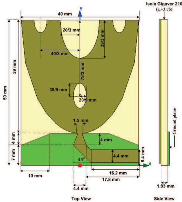
Fig. 10. Configuration of the UWB antenna (Al-Husseini et al., 2009)
