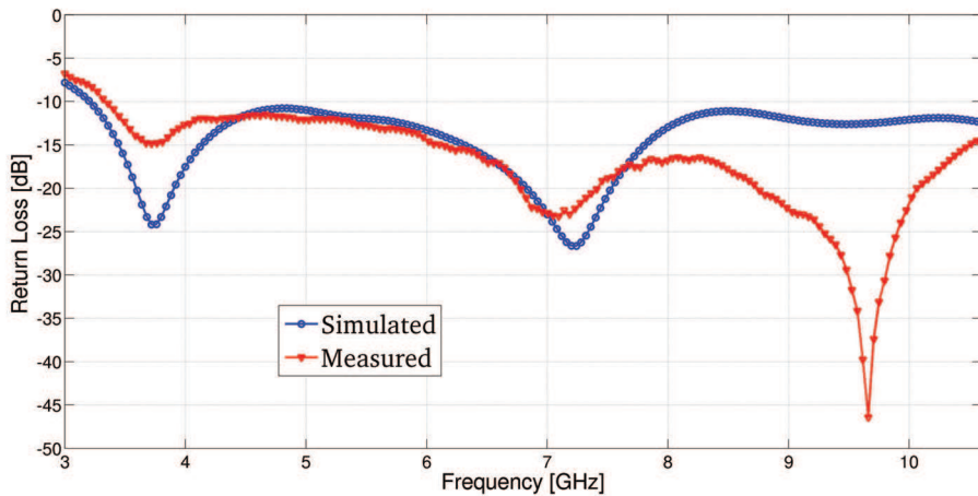
Fig. 7. Return loss of the sensing UWB antenna
