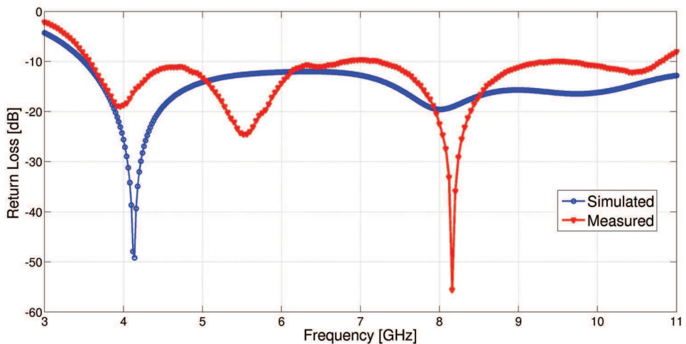
(b) Return loss without band notch
