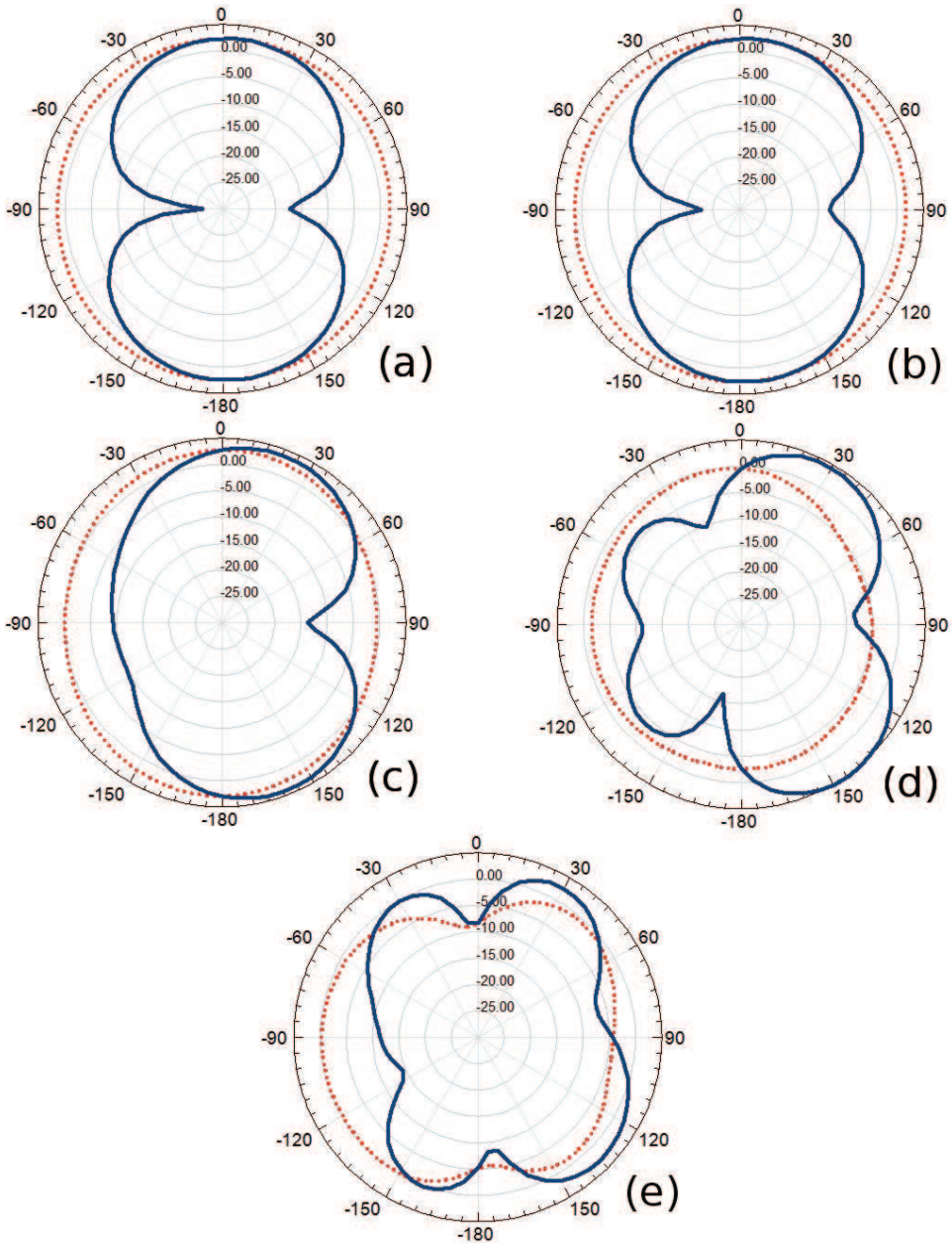
Fig. 12. Patterns in the X - Z plane (dotted line) and Y - Z plane (solid line) for (a) 2.1 GHz, (b) 2.4 GHz, (c) 3.5 GHz, (d) 5.1 GHz, and (e) 7 GHz (Al-Husseini et al., 2009)
