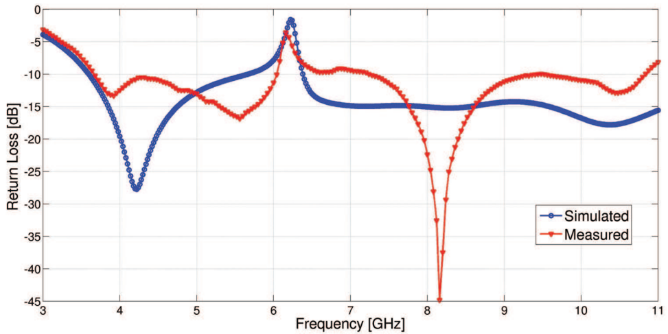
(a) Return loss with band notch
