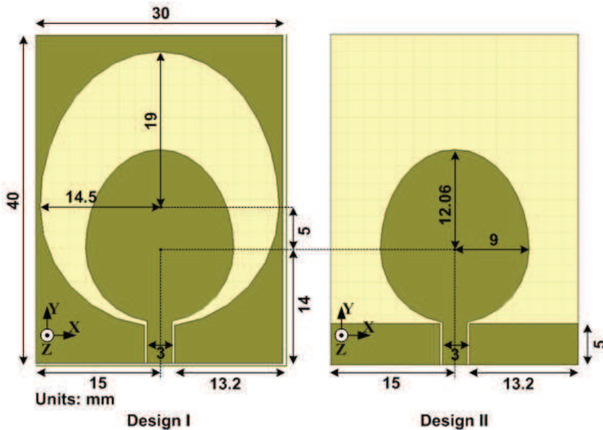
Fig. 9. Configuration of the two UWB designs (Al-Husseini et al., 2009a)
