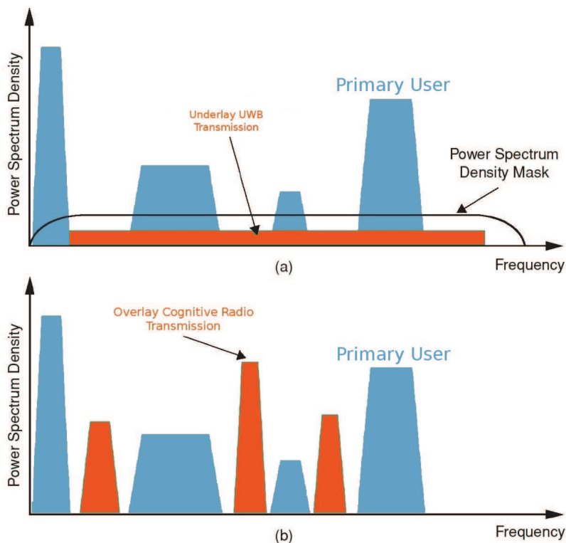
Fig. 3. Underlay (a) and overlay (b) spectrum sharing approaches
