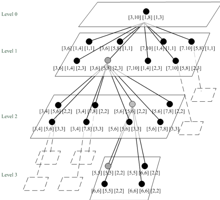
Fig. 3. A Constraint Tree for P2P mixer
