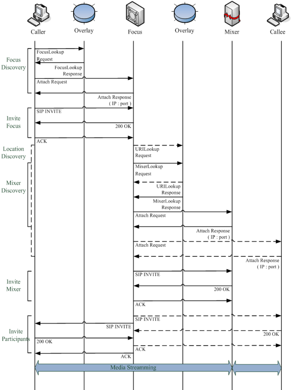
Fig. 6. The message sequence chart of a P2P-SIP conference setup
