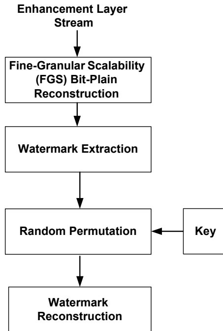
Fig. 7. Extracting a watermark from an Enhancement Layer of the MPEG-4 Fine Granularity Scalability (FGS) video stream (Wang et al., 2006).
