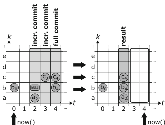
Fig. 9 Incremental commits
