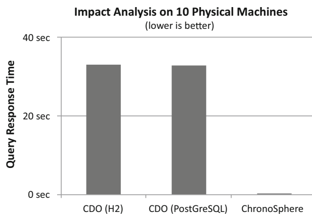
Fig. 24 Impact analysis performance
