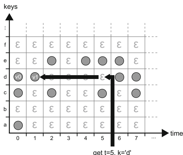
Fig. 4 A get operation on a Temporal Data Matrix [25]
