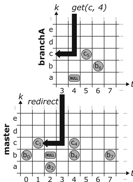
Fig. 7 Querying data stored in branches
