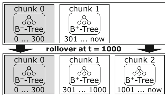
Fig. 10 The temporal rollover process by example [26]
