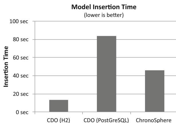
Fig. 21 Insertion performance
