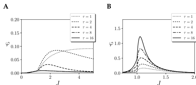
Figure 4. Integration of the cause repertoire \varphi_{\text{cause}}(\tau) of the largest mechanism of a homogeneous Ising model with one region of size N = 256 and couplings J with different temporal spans \tau , assuming (A) an independent prior and (B) the stationary distribution as a prior. Continuous noise injection is assumed.
