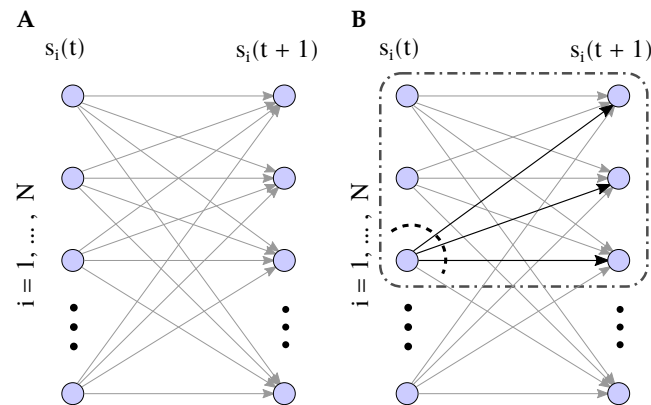
Figure 1. (A) Description of the infinite size kinetic Ising model. (B) Description of the partition schema used to define perturbations. Partitioned connections (black arrows) are injected with random noise. Nonpartitioned connections operate normally or are independent sources of noise (see Section 3.4).
