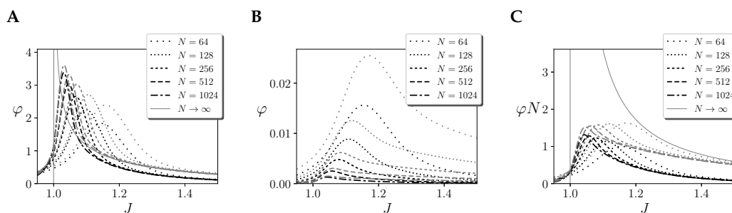
Figure 5. Integrated information \varphi(\tau) for the cause (black lines) and effect (grey lines) repertoires of the largest mechanism of a homogeneous kinetic Ising models with one region of size N (and infinite size when N \rightarrow \infty ) and coupling J using (A) the Wasserstein distance, (B) The Kullback–Leibler divergence, and (C) values of \varphi N using the Kullback–Leibler divergence. Note that in all cases \varphi(\tau) = \varphi_{\text{cause}}(\tau) . All cases are computed with \tau = 10 \log_2 N for finite systems and \tau \rightarrow \infty for infinite systems. Continuous noise injection and a stationary prior are assumed.
