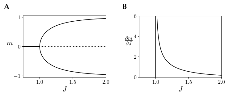
Figure 2. Description of the behaviour of the homogeneous Ising model with one region and coupling J , showing a critical point at J = 1 . (A) Values of mean firing rate m for the stationary solution of the kinetic Ising model with one homogeneous region. (B) Value of \frac{\partial m}{\partial J} for the positive stationary solution of the kinetic Ising model with one homogeneous region, diverging at the critical point.
