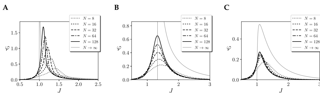
Figure 6. Effects of the environment in integrated information. Integrated information \varphi_{\mathcal{M}}(\tau) (black lines) of a mechanism \mathcal{M} of size \frac{3N}{4} of a homogeneous kinetic Ising model with one region of size N and coupling J , assuming that elements outside of the mechanism operate (A) normally, (B) as independent sources of noise and (C) as static input fields. Values of \varphi_{\mathcal{M}}(\tau) are compared with \varphi_{\mathcal{M},\text{effect}}(\tau \rightarrow \infty) (grey line) to show diverging tendencies of the effect repertoire. Note that tendencies of \varphi_{\mathcal{M},\text{effect}}(\tau \rightarrow \infty) are larger than values of \varphi_{\mathcal{M}}(\tau) , as the effect repertoire tends to show larger values. Values of \varphi are computed with \tau = 10 \log_2 N for finite systems and \tau \rightarrow \infty for infinite systems. Continuous noise injection and a stationary prior are assumed.
