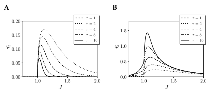
Figure 3. Integration of the effect repertoire \varphi_{\text{effect}}(\tau) of the largest mechanism of a homogeneous Ising model with one region of size N = 256 and couplings J with different temporal spans \tau , assuming (A) initial injection of noise and (B) continuous injection of noise. Note that \tau = 1 , in both cases \varphi_{\text{effect}} , has the same value.
