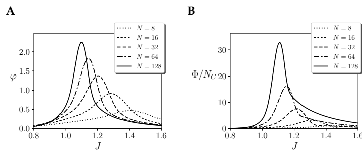
Figure 7. Mechanisms and system-level integration in a homogeneous system with one region of size N and coupling J . Values of (A) \varphi of the largest mechanism and (B) values of \Phi for the whole system. Measures with \tau = 10 \log_2 N , assuming continuous noise injection, stationary priors and environment coupling.
