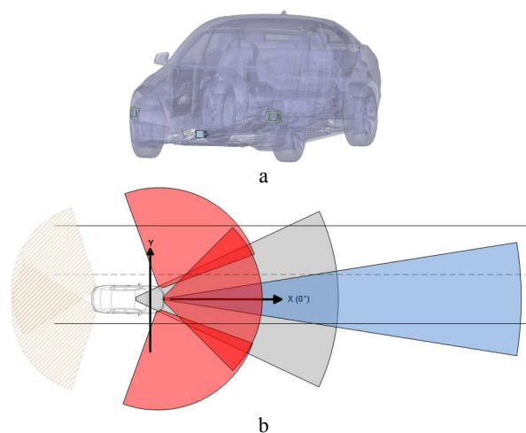
Fig. 7 Demonstrator car I - vehicle with functional setup: (a) Sensors integration site RADARS, (b) Radar sensor setup (3x Long Range Radar for VRU detection & classification >180°).
