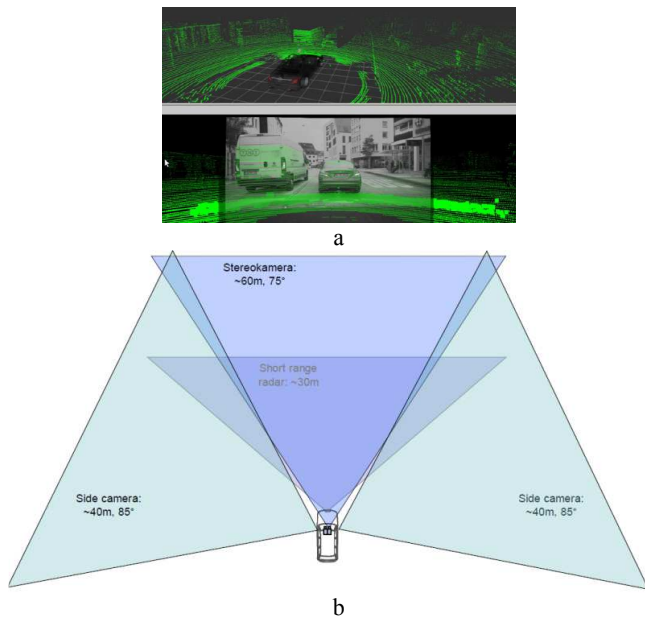
Fig. 8 Demonstrator car II: (a) Calibrated and synchronized stereo camera and lidar system, (b) Sensor setup consisting of one front facing stereo camera ( \sim 60\text{m} , 75^\circ ) and two side-oriented cameras covering a horizontal FOV of roughly 210^\circ .
