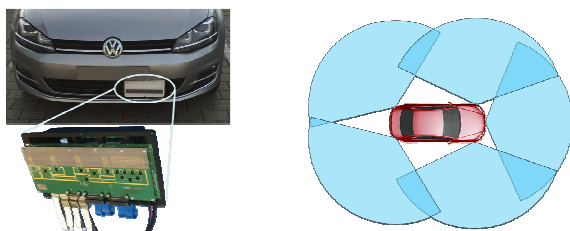
Fig. 9 Demonstrator car III - high resolution radar sensors: (a) Radar sensor mounting positions and FOV, (b) The demo-car equipped with radar sensor.
