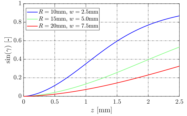
Figure 4: Scaling factor for F_s when Q is positive.
