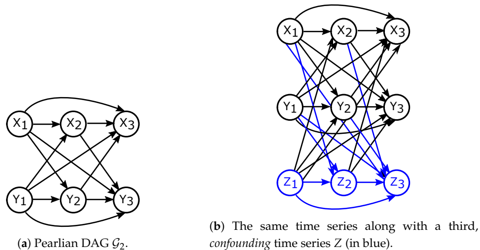
Figure 4. Pearlian DAGs representing partial ordering considered in Theorem 3.
