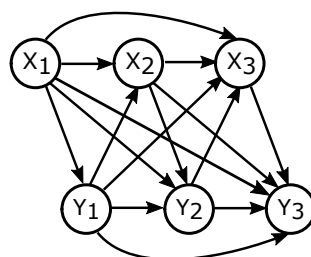
Figure 3. Pearlian DAG \mathcal{G}_1 representing full ordering considered in Theorem 2.
