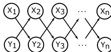
Figure 7. Example of “vanishing directed information” [28,29,82].
