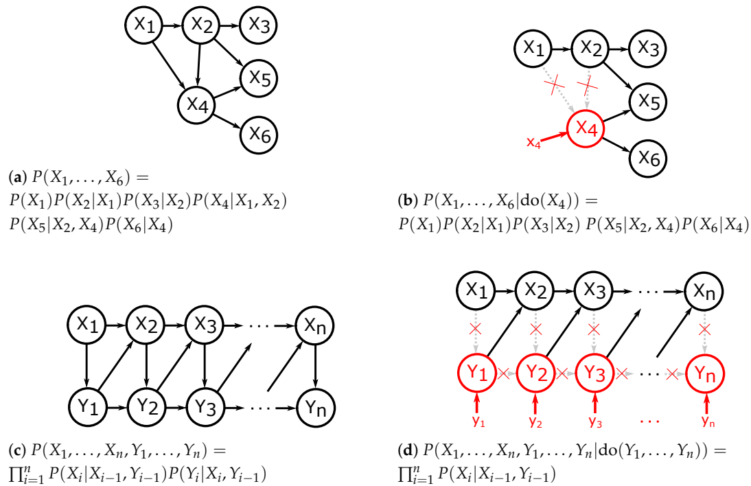
Figure 1. Examples of interventions performed on directed acyclic graphs (DAGs) with resulting probability factorisations. Left: observational distributions and factorisations. Right: interventional distributions and factorisations.
