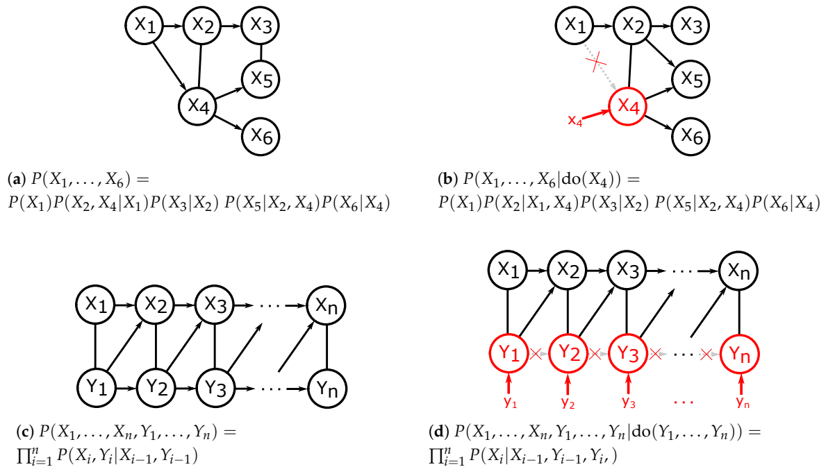
Figure 5. Examples of interventions performed on chain graphs with resulting probability factorisations. Left: observational distributions and factorisations. Right: interventional distributions and factorisations. Note that, as opposed to Figure 1, \{X_2, X_4\} (Figure 5a,b) and \{X_i, Y_i\} (Figure 5c,d) form chain components.
