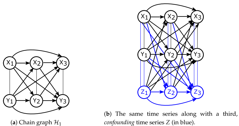
Figure 6. Chain graphs considered in Theorem 4.
