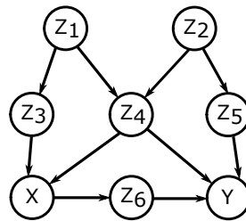
Figure 2. Adjustment sets for (X, Y) . Back-door adjustment [25]: \{Z_3, Z_4\} and \{Z_4, Z_5\} satisfy the back-door criterion with respect to (X, Y) . Only the former corresponds to adjusting for direct causes of X .
