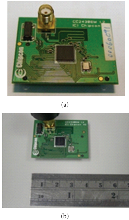
FIGURE 9: ZigBee evaluation module (EM) of CC2431ZDK.
