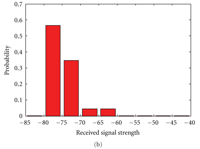
FIGURE 2: Histogram of probability of relative frequency (a) and RSS distribution (b).
