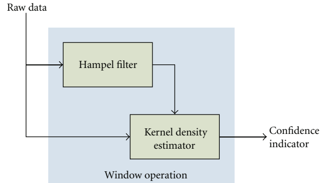
FIGURE 6: Proposed outlier detection scheme.
