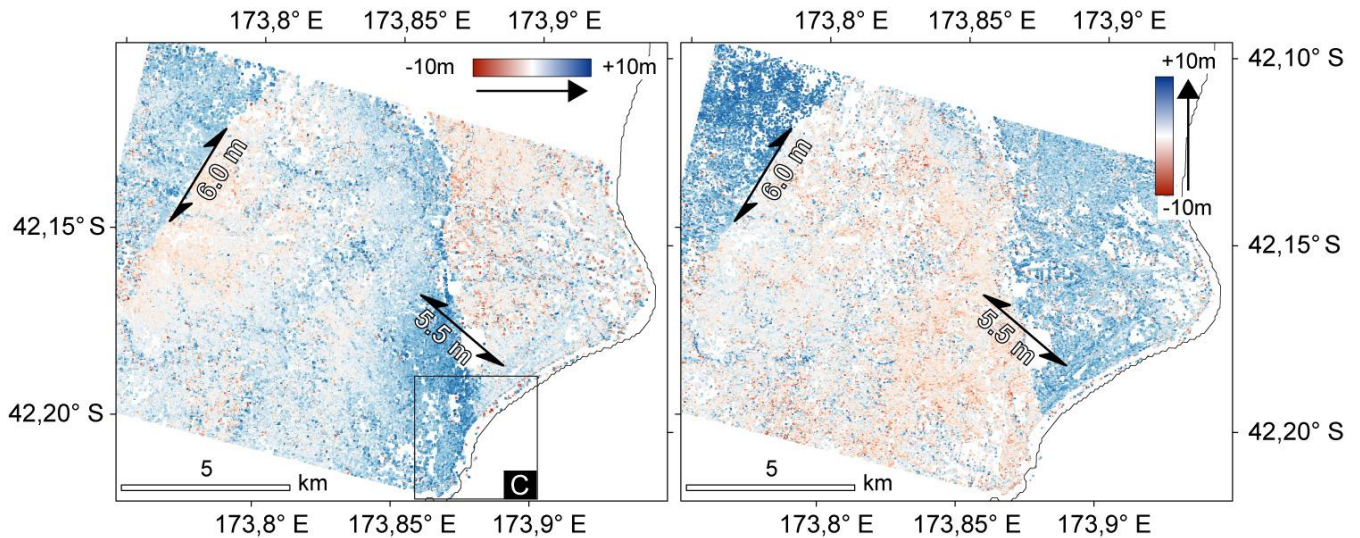
Figure 3: Horizontal surface displacements from PlanetScope images of 27 October – 28 November 2016. Left: W-E component, right: S-N component. Location: A in Fig. 2. The double arrows indicate the approximate direction and the according numbers the approximate magnitude of relative displacement over ruptures. Inset C: Fig. 5.
