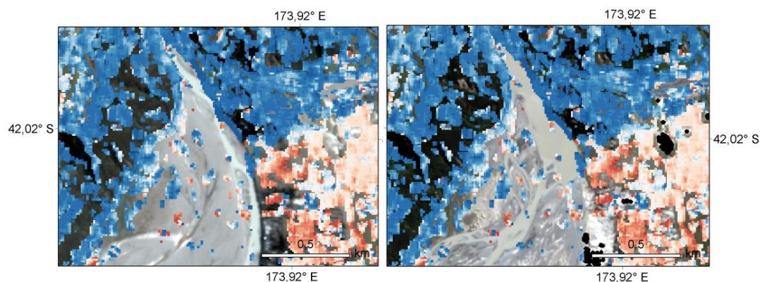
5 Figure 7: Horizontal surface displacements from PlanetScope images of 27 October – 21 November 2016, W-E component. Background: PlanetScope images of 27 October (left) and 21 November (right). Clarence River was dammed up by the rupture and its course diverted. Location: inset E of Fig. 4.
