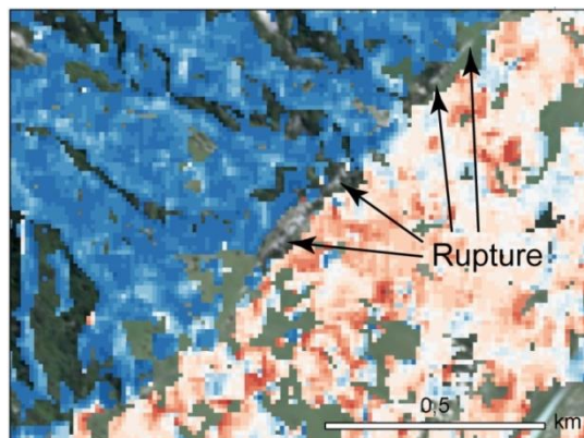
Figure 6: Horizontal surface displacements from PlanetScope images of 27 October – 21 November 2016, W-E component. Background: PlanetScope image of 21 November with the surface rupture well visible. Location: inset D of Fig. 4.
