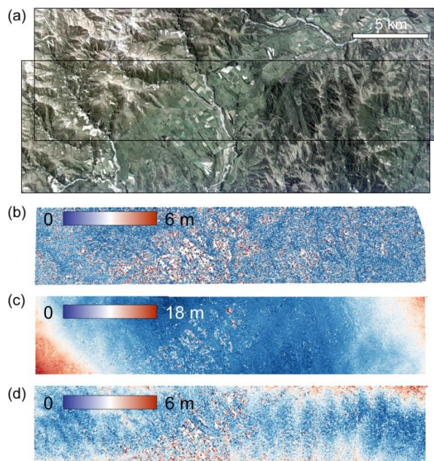
5 Figure 9: Horizontal surface displacements from PlanetScope images of 20 – 25 November 2016 without surface motion expected; total magnitude of displacement. (a) the two scenes and their overlap matched in panels (b)-(d). (b) displacements between orthorectified versions. (c) displacements between the unrectified versions, when co-registered by a 1 st -order polynomial. (d) like (c) but co-registered by 2 nd -order polynomial.
