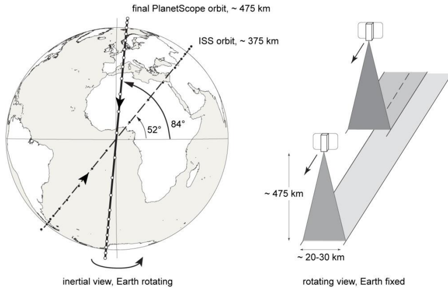
Figure 2: left panel: Final PlanetScope orbit and ISS test-bed orbit. Cubesat positions (white and black dots on the orbit) are only schematically indicated. The final PlanetScope orbit is planned to host over 100 cubesats. Right panel: scheme of complete scan of the Earth surface by successive PlanetScope cubesats in the same orbit.
