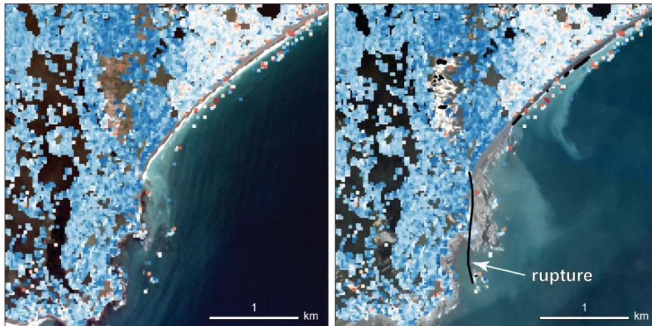
Figure 5: Horizontal surface displacements from PlanetScope images of 27 October – 21 November 2016, W-E component. Colorscale see Fig. 3. Left background: PlanetScope image of 27 October, right background 21 November 2016. The section of uplifted seabed (right of the rupture) and the according rupture are well visible in the PlanetScope images; the rupture is indicated by a black line that was digitized from the images. Location: C in Fig. 3.
