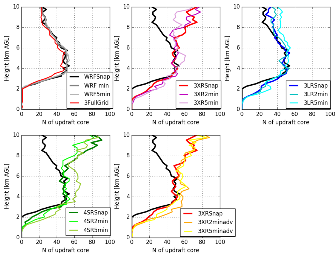
Figure 5: Vertical profiles of the number of coherent updrafts with vertical velocity > 5 \text{ m s}^{-1} . Colour represents different retrieval simulations as displayed in each panel. Dark gray line in (a) represents time average of the WRF output over 2 minutes from 12:18:00 to 12:19:40 UTC, and light gray in (a) represents time average of the WRF output over 5 min from 12:18:00 to 12:22:40 UTC. Each panel displays a profile from the WRF snapshot at 12:18:00 UTC by a black solid line.
