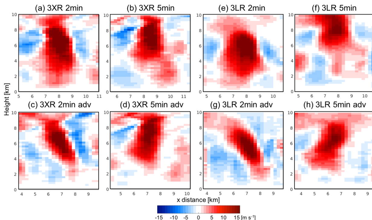
Figure 9: Vertical cross sections of vertical velocity for an updraft core from 3XR (a-d) and 3LR (e-h) wind retrieval simulations with 2-min and 5-min VCPs. Top row and bottom row display non-advection correction and advection-corrected retrievals, respectively. A selected updraft core is the
