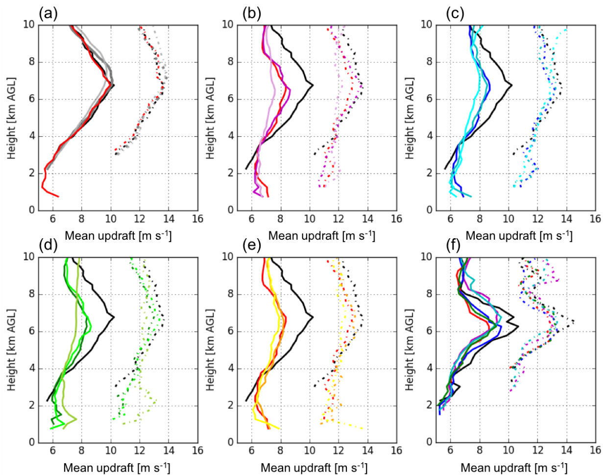
Figure 8: Same as Figure 7, but for mean updraft. Color representation is same as Figure 7.
