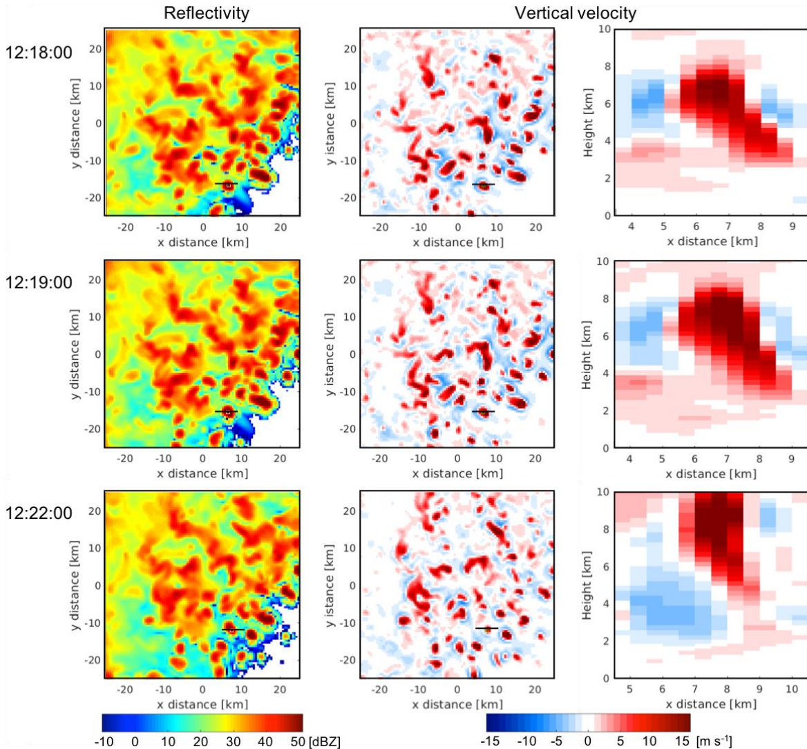
Figure 3: (Left column) Horizontal distributions of X-band radar reflectivity at 7 km AGL from CR-SIM, (middle column) horizontal distributions of the WRF simulated vertical velocity at 7 km 5 AGL, and (right column) vertical distributions of WRF-simulated vertical velocity along a line in the horizontal plots. Each row from top to bottom represents simulation time of 12:18:00, 12:19:00, and 12:22:00 UTC, respectively.
