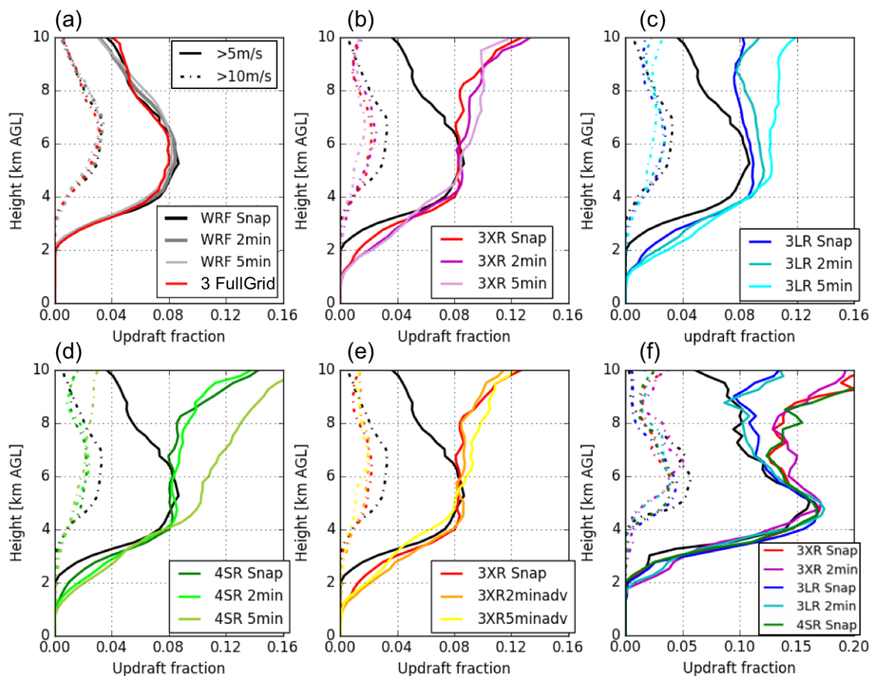
Figure 6: Vertical profiles of updraft fractions with different thresholds of 5 \text{ m s}^{-1} (solid lines) and 10 \text{ m s}^{-1} (dashed lines) for the entire retrieval domain (a – e) and a center region shown as a box in Fig. 2 (f). Color represents different retrieval simulations as displayed in each panel.
