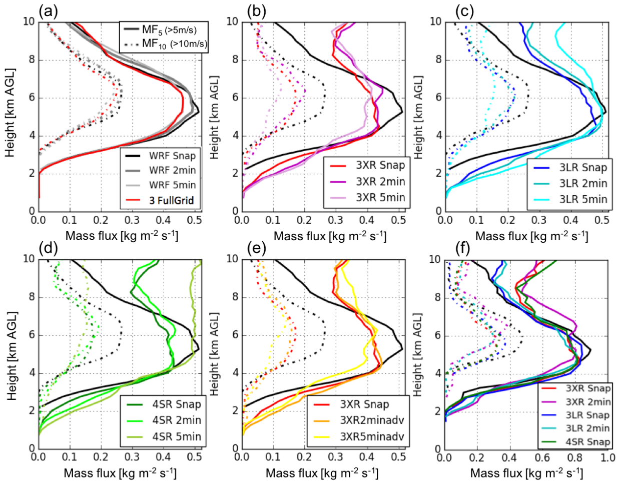
Figure 7: Vertical profiles of convective mass flux with different updraft thresholds of 5 \text{ m s}^{-1} (solid lines) and 10 \text{ m s}^{-1} (dashed lines) for the entire retrieval domain (a–e) and a center region shown as a box in Fig. 2 (f). Color represents different retrieval simulations as displayed in each panel.
