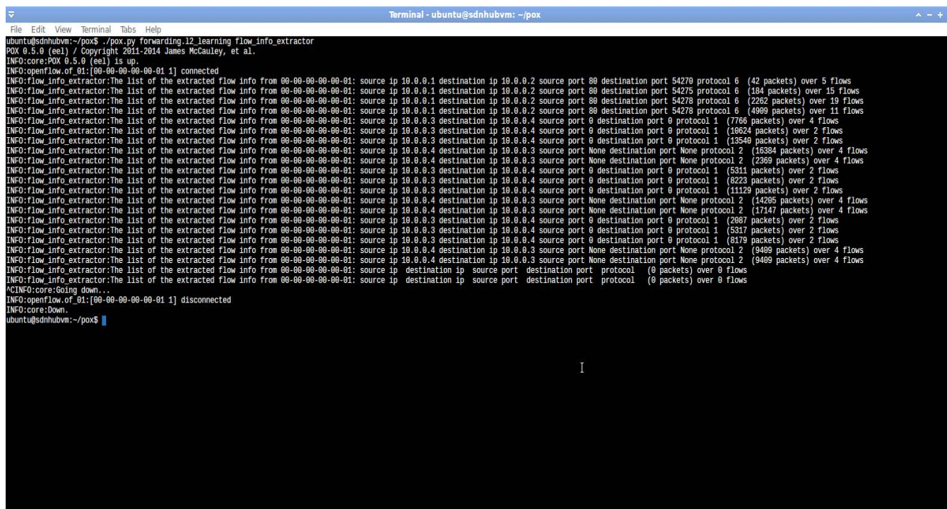
Fig. 4 Flow header information obtained by the POX controller module
