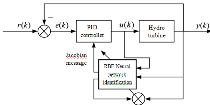
Fig.9. RBF - PID controller design
