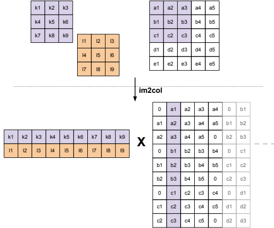
Figure 1. GEMM input preparation: im2col transformation applied to two 3×3 kernels and portion of the larger input matrix generated from the smaller original 5×5 input image.
