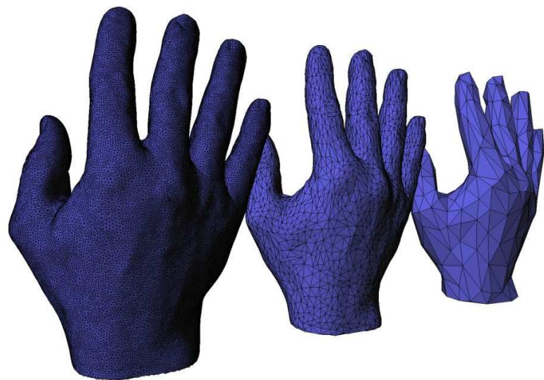
Figure 7.16: A variety of mesh simplification algorithms can be used to reduce the model complexity while retaining the most important structures. Shown here is a simplification of a hand model made by the open-source library CGAL. (Figure by Fernando Cacciola.)
