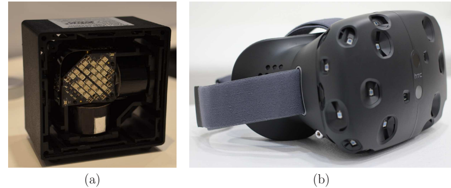
Figure 9.16: The laser-based tracking approach used in the HTC Vive headset: (a) A base station contains spinning drums that emit horizontal and vertical sheets of IR light. An array of IR LEDs appears in the upper left, which provide a synchronization flash (photographer Ben Lang, publisher: Road to VR). (b) Photodiodes in pockets on the front of the headset detect the incident IR light (photo by Maurizio Pesce, CC BY 2.0).
