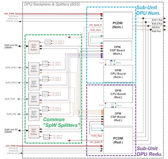
Fig. 28. Schematic of the SWA-DPU hardware architecture
