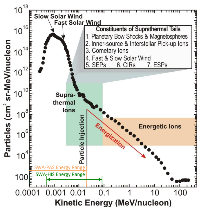
Fig. 2. SWA measurement range for the ion composition and energy distribution extending from the solar wind into the supra-thermal domain and covering the energy range of SEP seed particles injected to shock acceleration (adapted from Mewaldt et al. (2003); shown here are oxygen fluences from ACE measured over a 3-year period). SWA-PAS and SWA-HIS energy ranges are shown at the bottom of the figure for comparison.
