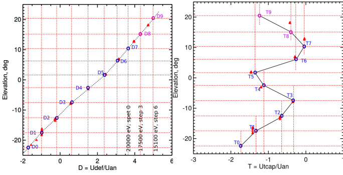
Fig. 25. SWA-PAS optimisation results that provide the basis for FPGA sequencer code inputs. The left panel shows the variation of the elevation angle as a function of the ratio between the voltage on the deflector (Udef) and that on the analyser (Uan), while the right panel shows the variation of the elevation angle as a function of the ratio between the voltage on the top cap (Utcap) and Uan.
