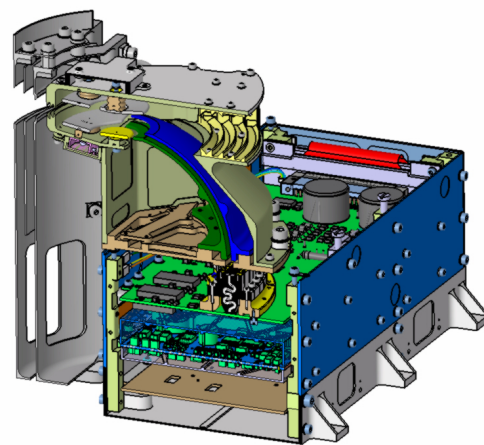
Fig. 17. Three-dimensional cut of the full SWA-PAS instrument illustrating the three main elements of SWA-PAS design: 1) The analyser (sensor head); 2) The electronics box containing the CEM detectors, HV sources, and other electronics boards; 3) The front thermal shield.
