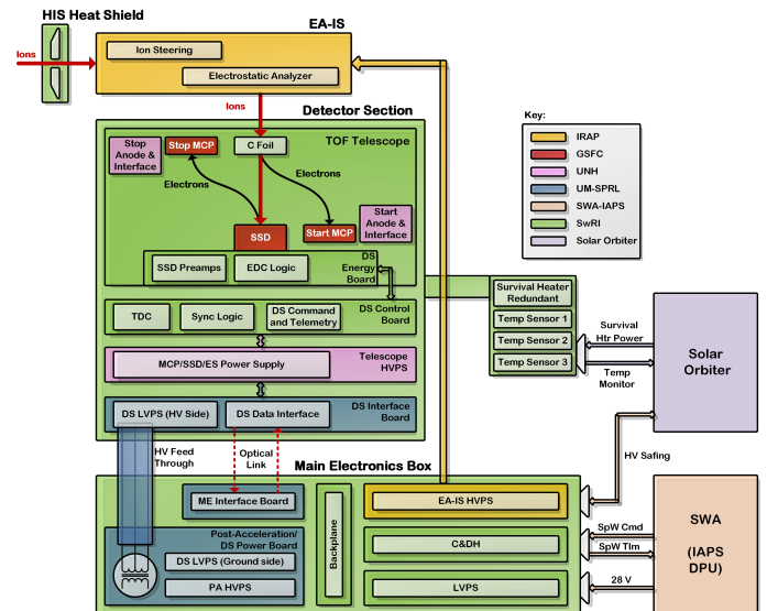
Fig. 12. HIS block diagram
