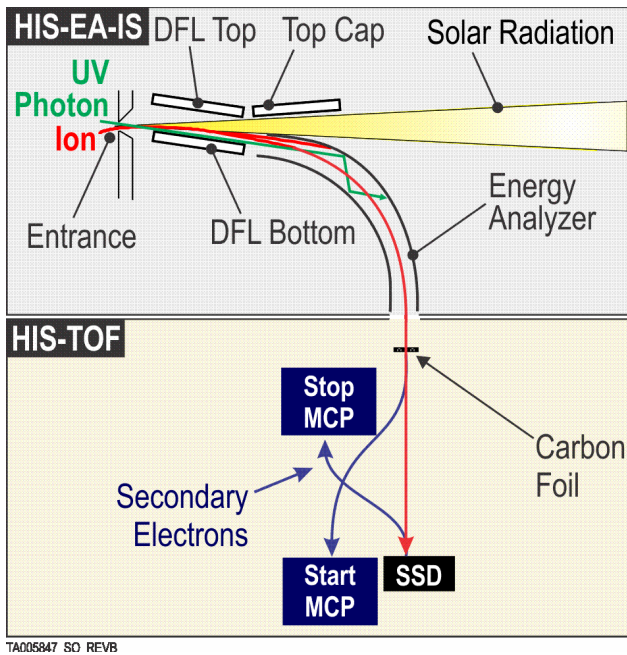
Fig. 11. Schematic of SWA-HIS with example particle trajectory. The cut-plane for the top part of the figure is that containing the Sun-spacecraft line and the direction of elevation deflection. The yellow shading represents the passage of direct solar light through the sensor and the red curve indicates a representative ion trajectory in this plane. The instrument has partial cylindrical symmetry extending from -33^\circ to +66^\circ out of the plane of the figure.
