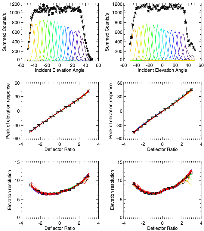
Fig. 9. Elevation response of FM SWA-EAS sensors heads (SWA-EAS1 in left column, SWA-EAS2 in right column). Top row shows the counts received in each sensor elevation bin as a function of the elevation angle of the incident electron beam. The second row shows the elevation angle showing peak response as a function of the voltage ratio applied to the deflectors, showing good linearity. The bottom row shows the FWHM of the response angle as a function of the voltage ratio, indicating that there is an asymmetry in the response for ‘upward’ and ‘downward’ sweeps and that the acceptance angle is larger at larger deflections.
