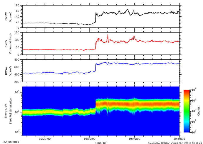
Fig. 34. Simulation of a SWA-PAS Energy-Time Spectrogram: Three top panels: The input parameters to the simulation as measured by the BMSW instrument onboard the RadioAstron mission. Bottom panel: Expected sensor response integrated over all angular bins. The time of the measurements is shifted relative to UT by about 1.5 hours.
