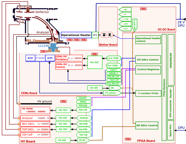
Fig. 21. Block Diagram of the SWA-PAS system.
