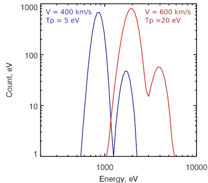
Fig. 35. Simulated examples of SWA-PAS energy spectra for different solar wind conditions. The temperature of He 2+ peak is assumed as T_p \times 4 .
