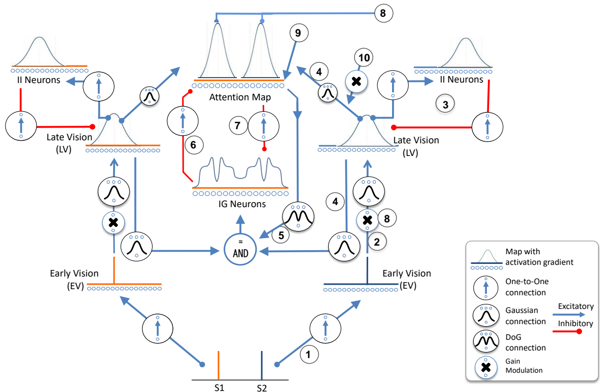
Figure 5. Illustration of the complete architecture for two distinct pathways during perception of two stimuli S1 and S2 with highly distinct dimensions (e.g. form vs color). The left and the right side represent the same connections but for different kinds of stimuli. The bubbles indicate the spatial distribution and character of each connection. The traces above each layer illustrate a typical activation profile for that map in response to a stimulus. Note that attention affects both pathways, regardless of which stimulus triggered it. The numbers correspond to descriptors in the text.
