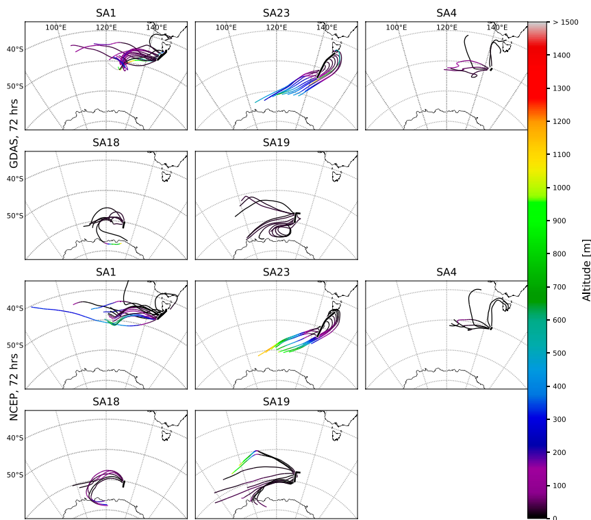
Fig. 4. Three-day back trajectories calculated using HYSPLIT and two different meteorological datasets (GDAS 1° and NCEP/NCAR reanalysis), initiated at each sampling date and location, and 25-m altitude.
