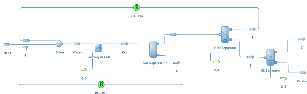
Figure 7. Simulation scheme for water electrolysis in DWSIM.
