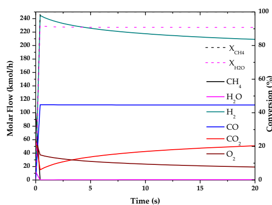
Figure 6. Evolution of molar flow profiles over time for Autothermal Reforming of Methane ( T = 1510\text{ K} ; P = 21\text{ bar} ). The figures show the final molar flow results for each component involved in the reactions and fuel conversion, both as a function of the residence time to equilibrium, or to a fixed time known by the reference used for its simulation.
