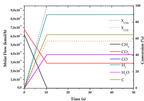
Figure 2. Evolution of molar flow profiles over time for Dry Reforming of Methane ( T = 973 \text{ K} ; P = 1 \text{ bar} ).
