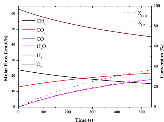
Figure 4. Evolution of molar flow profiles over time for Partial Oxidation of Methane ( T = 1223\text{ K} ; P = 1\text{ bar} ).
