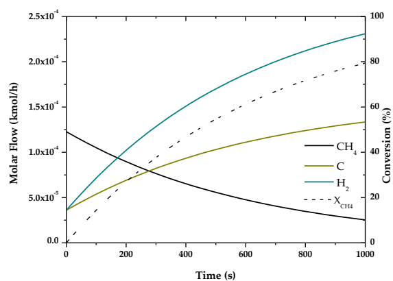
Figure 1. Evolution of molar flow profiles over time for Natural Gas Pyrolysis ( T = 1173 \text{ K} ; P = 1 \text{ bar} ).
