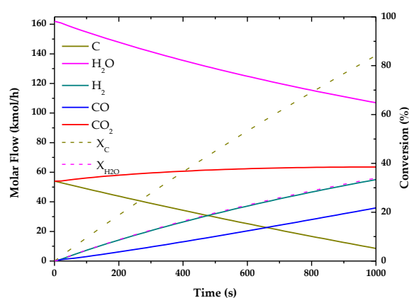
Figure 5. Evolution of molar flow profiles over time for Coal Gasification ( T = 1123\text{ K} ; P = 1\text{ bar} ).
