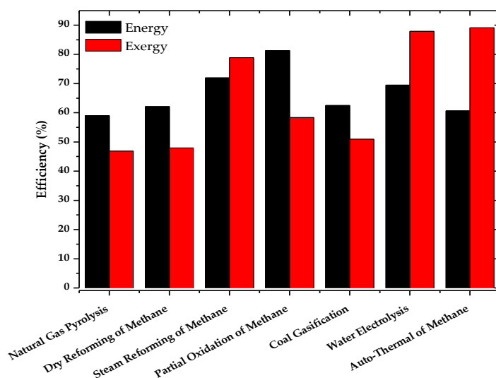
Figure 8. Comparison between energy and exergy efficiencies.
