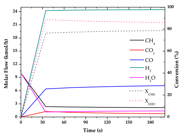
Figure 3. Evolution of molar flow profiles over time for Steam Reforming of Methane ( T = 1000 \text{ K} ; P = 1 \text{ bar} ).
