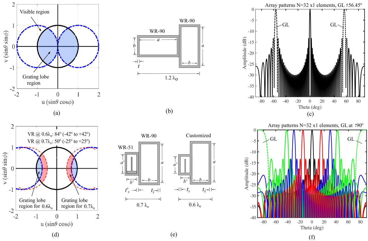
FIGURE 1: Grating lobe diagram using a conventional and proposed compact waveguide unit cell for dual-polarized array antenna. In (a-b) Grating lobe and dual-polarized unit cell based on conventional WR-90 waveguides, in this case unit cell spacing is 1.2\lambda_0 . (c) Array antenna pattern of 32x1 linear array with spacing of 1.2\lambda_0 . In (d-e) Grating lobe analysis for a dual-polarized unit cell based on proposed compact waveguides using standard waveguides; WR-51 for V-pol and WR-90 for H-pol for 0.7\lambda_0 and 0.6\lambda_0 . (f) Array antenna pattern of 32x1 linear array with spacing of 0.6\lambda_0 . Grating lobe only appears after e-scanning is larger than \pm 42^\circ .
