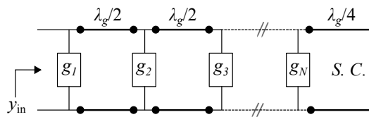
FIGURE 3: The equivalent circuit model of resonant slotted waveguide antenna array with shunt conductances.
