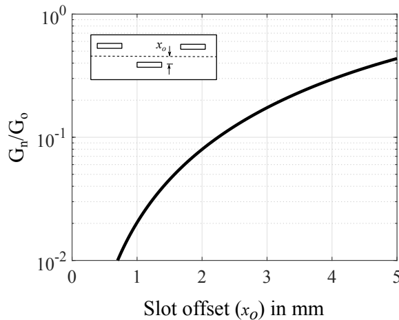
FIGURE 4: Normalized resonant conductance g_n(x_0) vs. slot offset x_0 of isolated longitudinal shunt slot in a WR-90 standard (with a = 22.86 mm and b = 10.16 mm) at 9.4 GHz.
