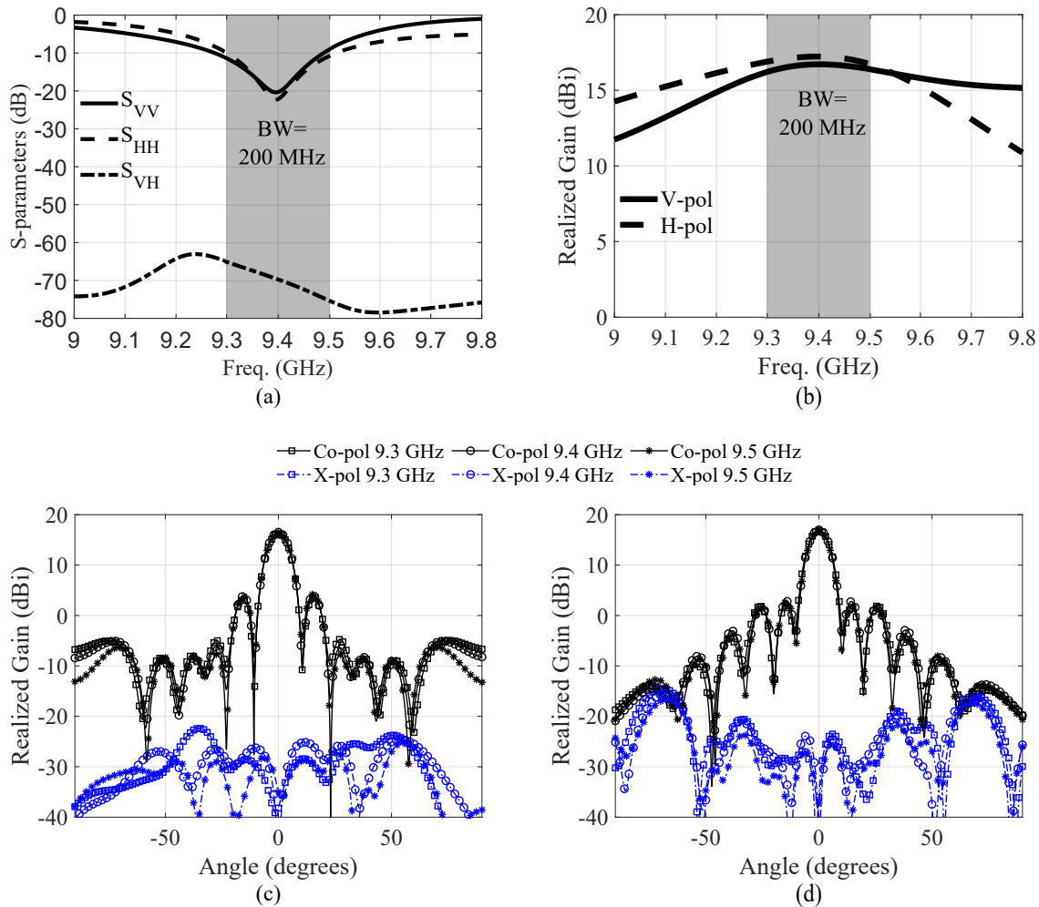
FIGURE 7: (a) S-parameters of the proposed dual-polarization antenna (b) Realized gain values versus the frequency for V-pol antenna and H-pol antenna (c) Co- and cross-pol gain radiation patterns at 9.3 GHz, 9.4 GHz and 9.5 GHz of H-pol antenna in the E-plane (d) Co- and cross-pol gain radiation patterns at 9.3 GHz, 9.4 GHz and 9.5 GHz of V-pol antenna in the H-plane.
