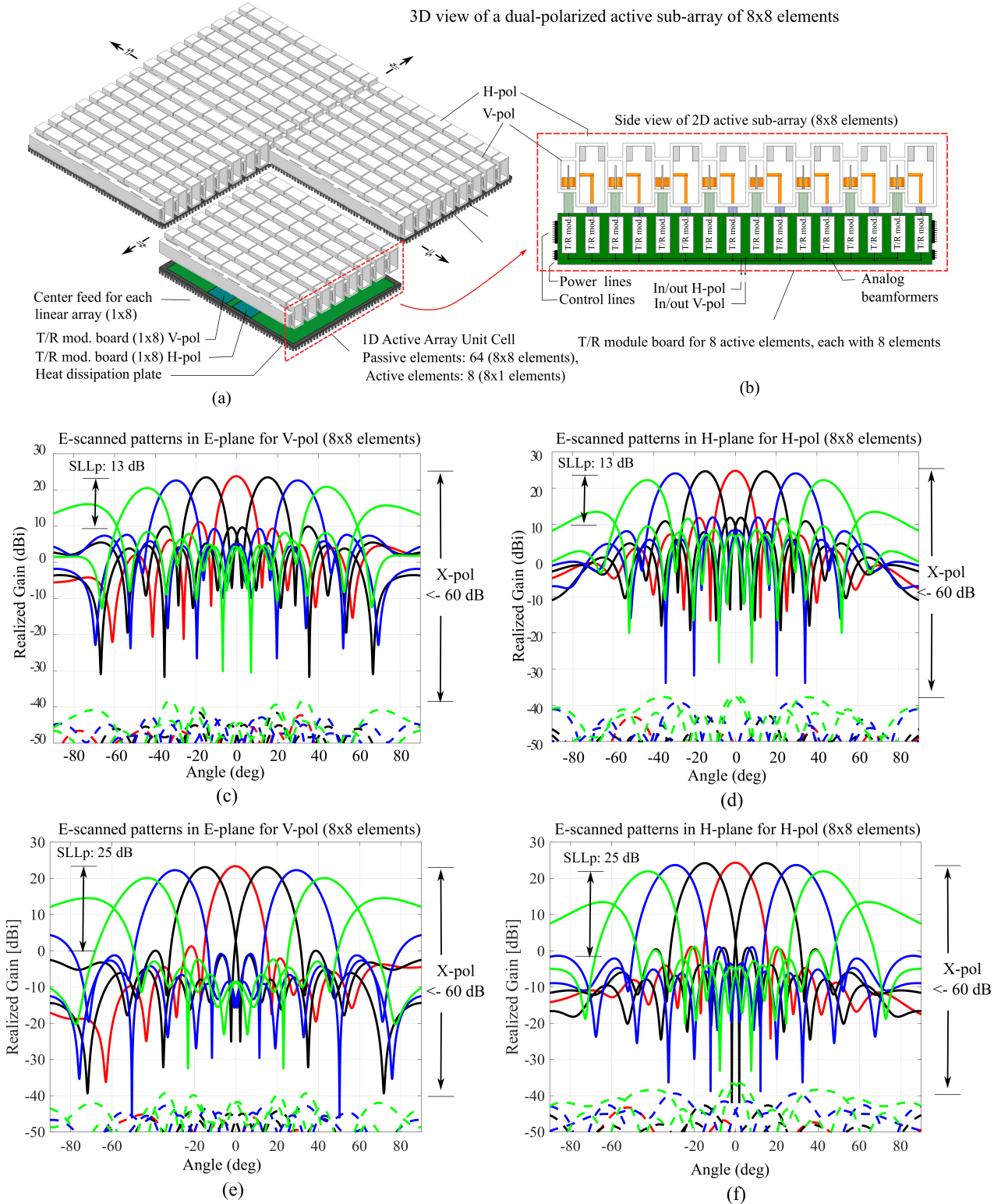
FIGURE 8: Geometry of proposed active dual-polarized planar SWGA array (a) 3D view; (b) Side view of the feeding structure. Simulated co- and cross-polarization patterns scanning characteristics at 9.4 GHz at various scan angles \theta_s = \pm 0^\circ, \pm 15^\circ, \pm 30^\circ, \pm 45^\circ (c) E-plane of V-polarization antenna with uniform illumination; (d) H-plane of H-polarization antenna with uniform illumination (e) E-plane of V-polarization antenna with tapered illumination; (f) H-plane of H-polarization antenna with tapered illumination.
