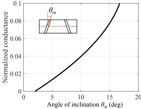
FIGURE 5: The variation of the normalized conductance with the angle of inclination of shunt slot in the narrow wall of a WR-90 with a = 22.86 mm and b = 10.16 mm at 9.4 GHz.
