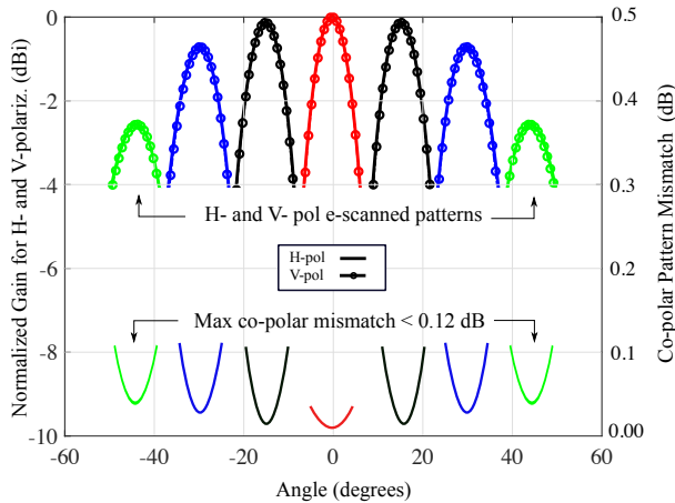
FIGURE 9: Simulated co-polar patterns mismatch at 9.4 GHz with uniform illumination at various scan angles \theta_s = \pm 0^\circ, \pm 15^\circ, \pm 30^\circ, \pm 45^\circ .
